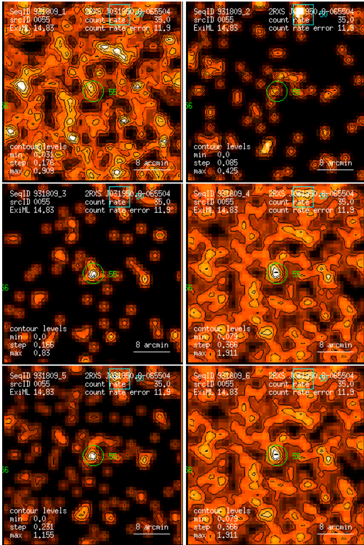
Figure 55: RASS 931809: detection 0055: band rate images, Gaussian filter: (1) PSPC channels 11 – 41, (2) 52 – 90, (3) 91 – 201, (4) 11 – 235, (5) 52 – 201, (6) 11 – 201. Broad band rates in counts/ks. Band rate contour levels in counts/ks/arcmin 2 .
