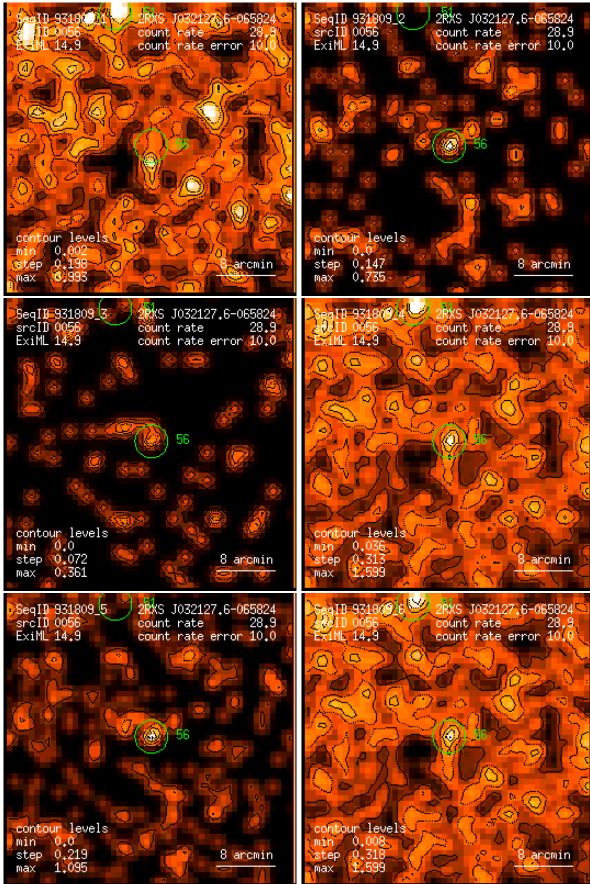
Figure 56: RASS 931809: detection 0056: band rate images, Gaussian filter: (1) PSPC channels 11 – 41, (2) 52 – 90, (3) 91 – 201, (4) 11 – 235, (5) 52 – 201, (6) 11 – 201. Broad band rates in counts/ks. Band rate contour levels in counts/ks/arcmin 2 .
