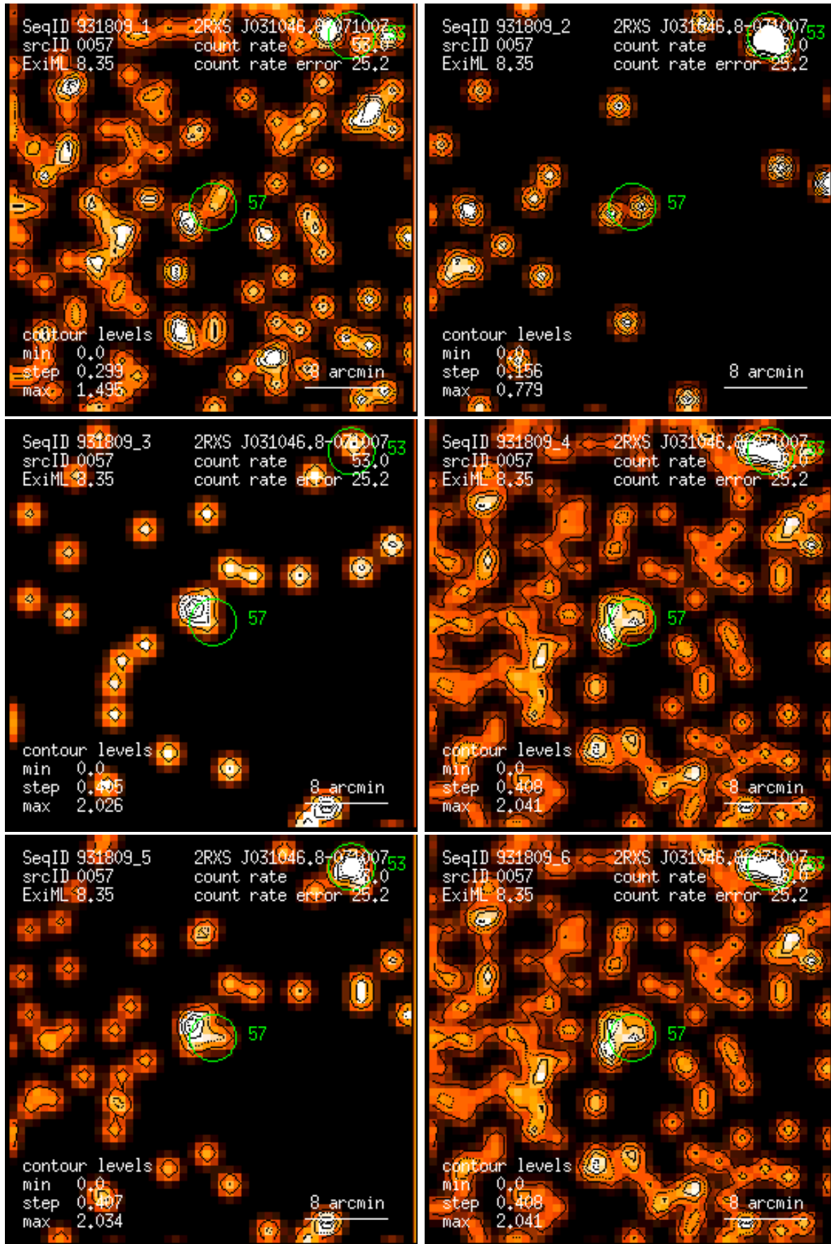
Figure 57: RASS 931809: detection 0057: band rate images, Gaussian filter: (1) PSPC channels 11 – 41, (2) 52 – 90, (3) 91 – 201, (4) 11 – 235, (5) 52 – 201, (6) 11 – 201. Broad band rates in counts/ks. Band rate contour levels in counts/ks/arcmin 2 .
