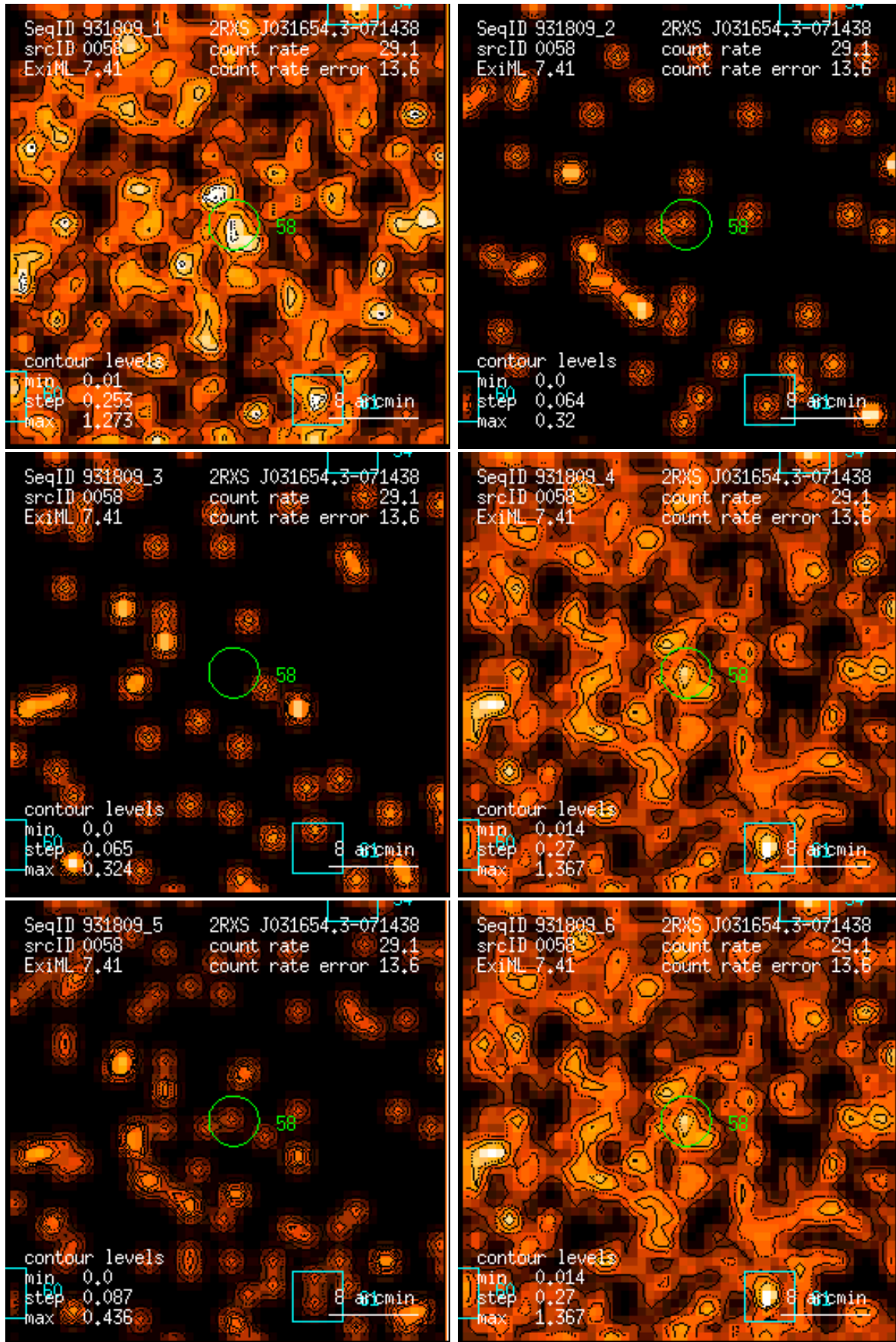
Figure 58: RASS 931809: detection 0058: band rate images, Gaussian filter: (1) PSPC channels 11 – 41, (2) 52 – 90, (3) 91 – 201, (4) 11 – 235, (5) 52 – 201, (6) 11 – 201. Broad band rates in counts/ks. Band rate contour levels in counts/ks/arcmin 2 .
