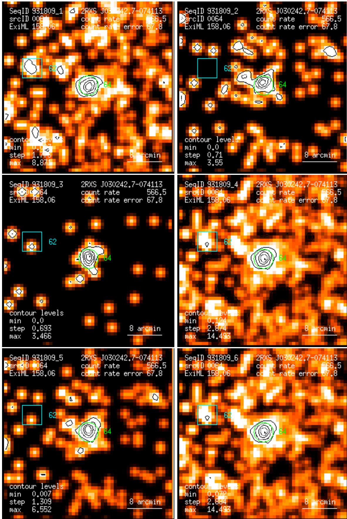
Figure 64: RASS 931809: detection 0064: band rate images, Gaussian filter: (1) PSPC channels 11 – 41, (2) 52 – 90, (3) 91 – 201, (4) 11 – 235, (5) 52 – 201, (6) 11 – 201. Broad band rates in counts/ks. Band rate contour levels in counts/ks/arcmin 2 .
