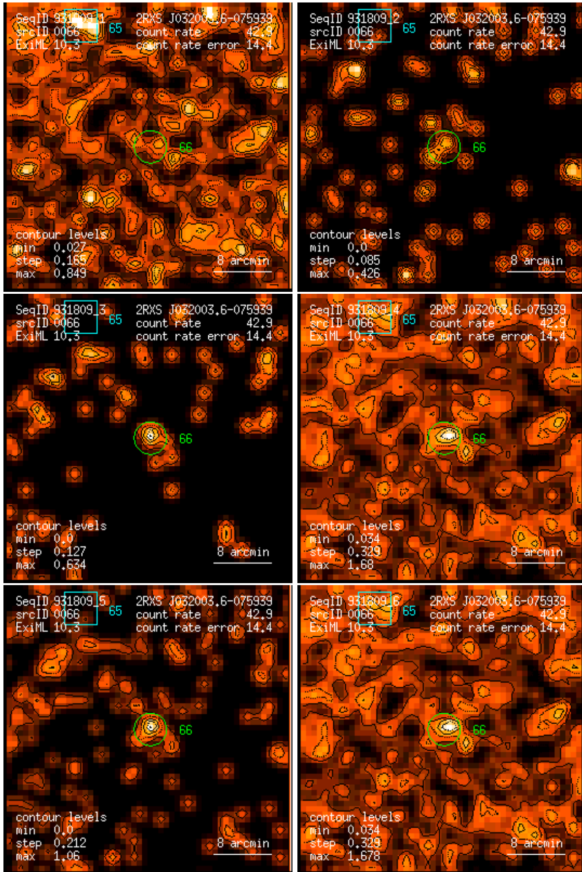
Figure 66: RASS 931809: detection 0066: band rate images, Gaussian filter: (1) PSPC channels 11 – 41, (2) 52 – 90, (3) 91 – 201, (4) 11 – 235, (5) 52 – 201, (6) 11 – 201. Broad band rates in counts/ks. Band rate contour levels in counts/ks/arcmin 2 .
