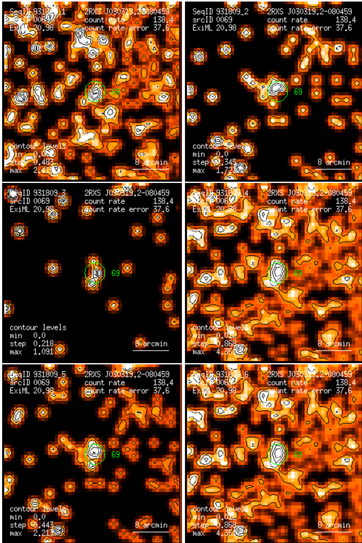
Figure 69: RASS 931809: detection 0069: band rate images, Gaussian filter: (1) PSPC channels 11 – 41, (2) 52 – 90, (3) 91 – 201, (4) 11 – 235, (5) 52 – 201, (6) 11 – 201. Broad band rates in counts/ks. Band rate contour levels in counts/ks/arcmin 2 .
