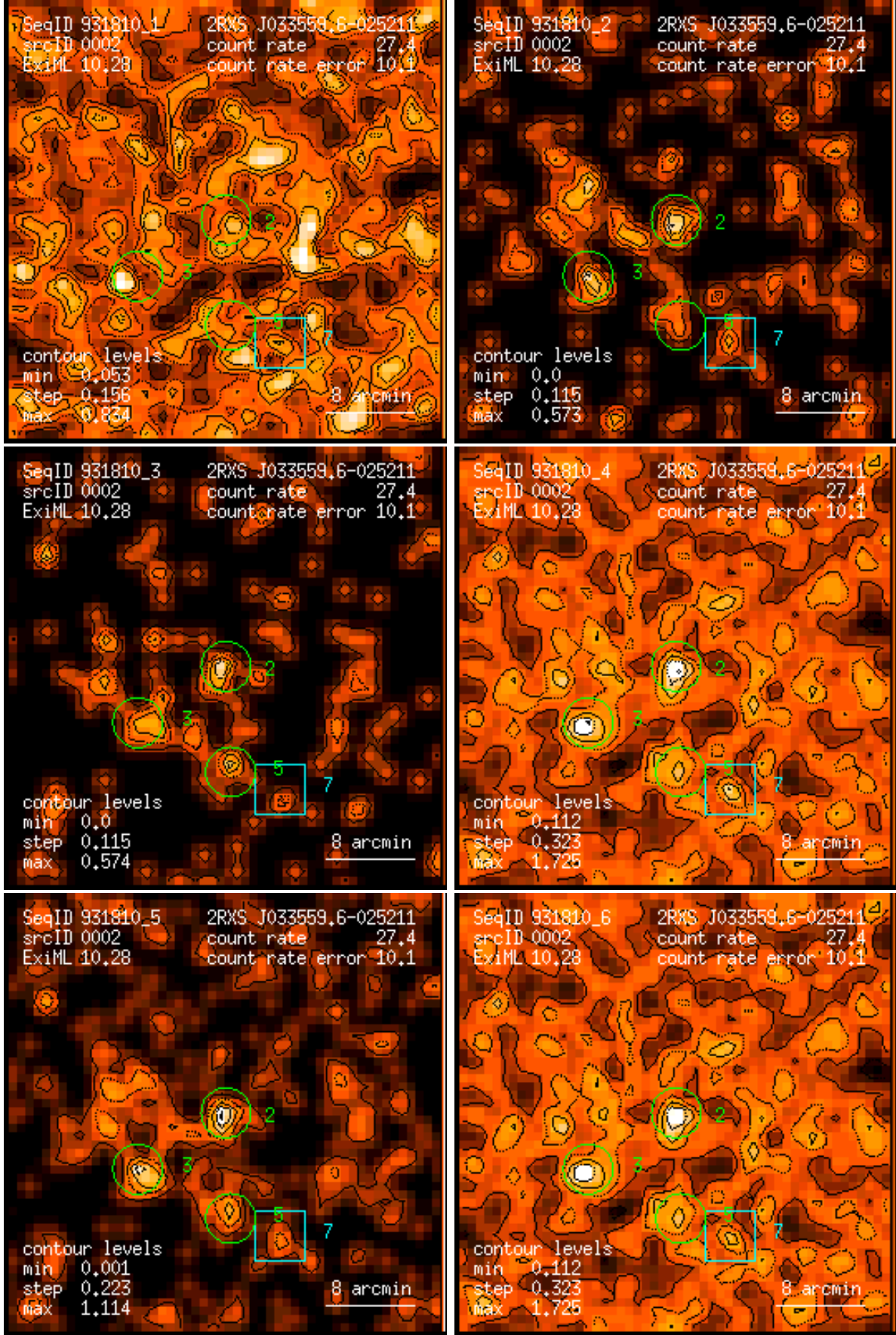
Figure 2: RASS 931810: detection 0002: band rate images, Gaussian filter: (1) PSPC channels 11 – 41, (2) 52 – 90, (3) 91 – 201, (4) 11 – 235, (5) 52 – 201, (6) 11 – 201. Broad band rates in counts/ks. Band rate contour levels in counts/ks/arcmin 2 .
