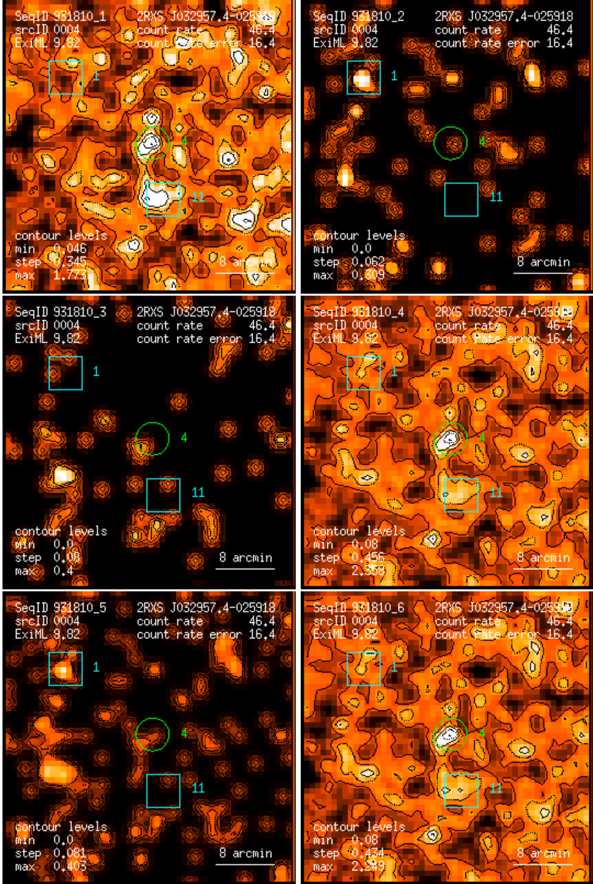
Figure 4: RASS 931810: detection 0004: band rate images, Gaussian filter: (1) PSPC channels 11 – 41, (2) 52 – 90, (3) 91 – 201, (4) 11 – 235, (5) 52 – 201, (6) 11 – 201. Broad band rates in counts/ks. Band rate contour levels in counts/ks/arcmin 2 .
