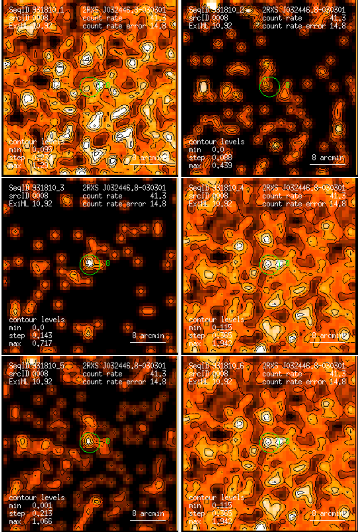
Figure 8: RASS 931810: detection 0008: band rate images, Gaussian filter: (1) PSPC channels 11 – 41, (2) 52 – 90, (3) 91 – 201, (4) 11 – 235, (5) 52 – 201, (6) 11 – 201. Broad band rates in counts/ks. Band rate contour levels in counts/ks/arcmin 2 .
