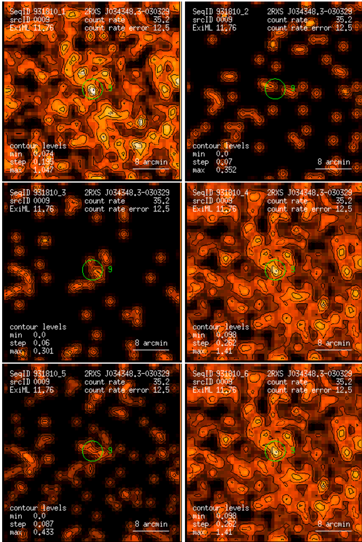
Figure 9: RASS 931810: detection 0009: band rate images, Gaussian filter: (1) PSPC channels 11 – 41, (2) 52 – 90, (3) 91 – 201, (4) 11 – 235, (5) 52 – 201, (6) 11 – 201. Broad band rates in counts/ks. Band rate contour levels in counts/ks/arcmin 2 .
