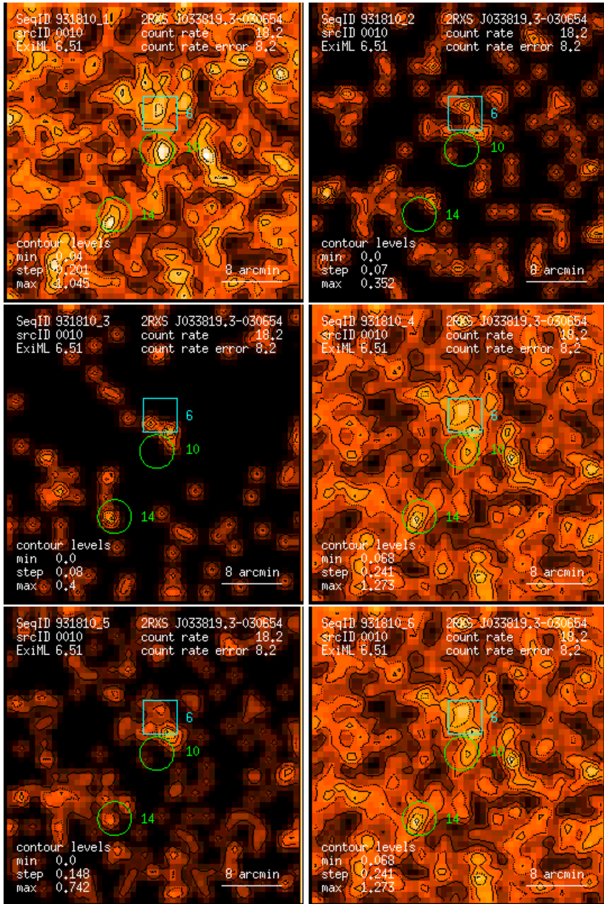
Figure 10: RASS 931810: detection 0010: band rate images, Gaussian filter: (1) PSPC channels 11 – 41, (2) 52 – 90, (3) 91 – 201, (4) 11 – 235, (5) 52 – 201, (6) 11 – 201. Broad band rates in counts/ks. Band rate contour levels in counts/ks/arcmin 2 .
