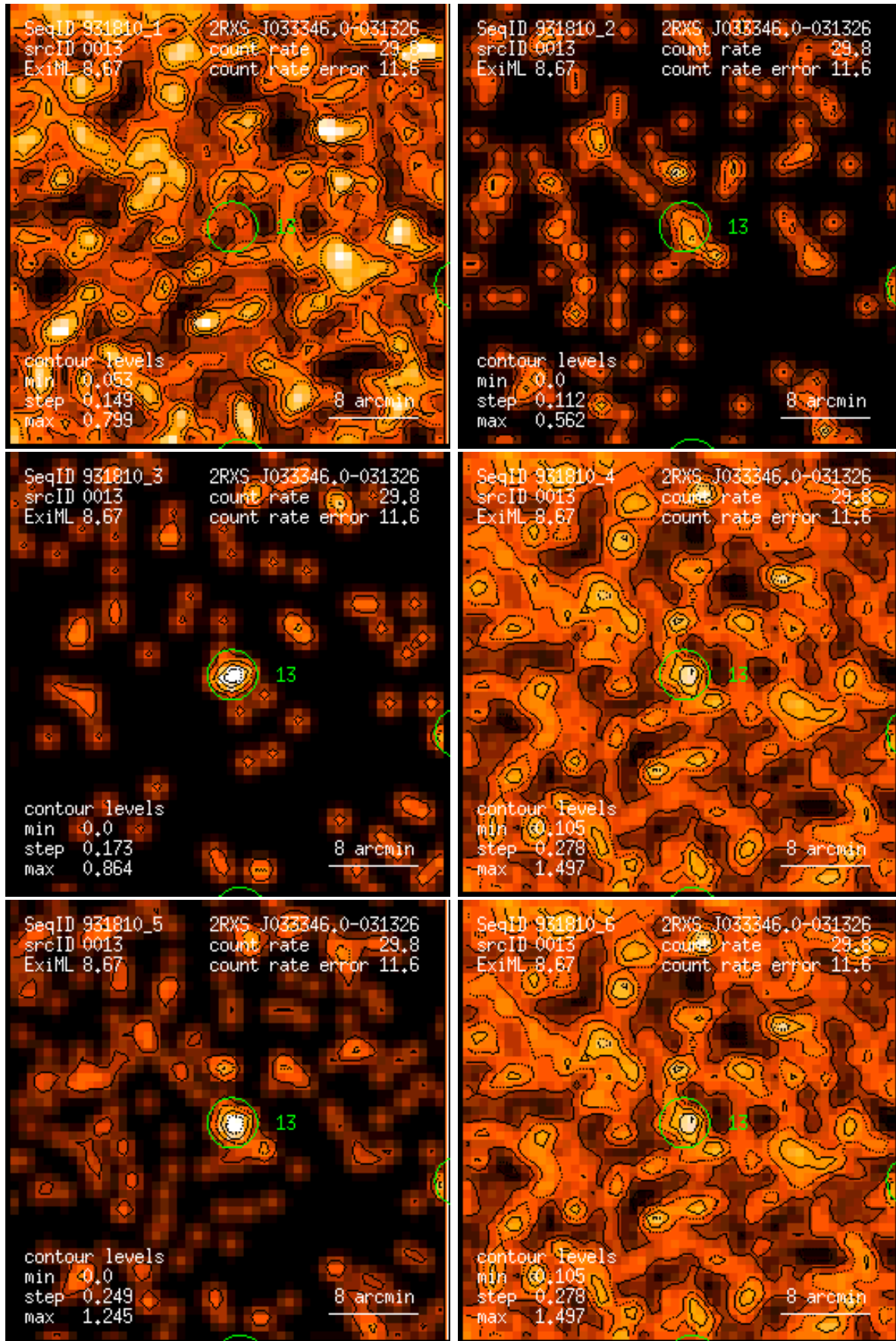
Figure 13: RASS 931810: detection 0013: band rate images, Gaussian filter: (1) PSPC channels 11 – 41, (2) 52 – 90, (3) 91 – 201, (4) 11 – 235, (5) 52 – 201, (6) 11 – 201. Broad band rates in counts/ks. Band rate contour levels in counts/ks/arcmin 2 .
