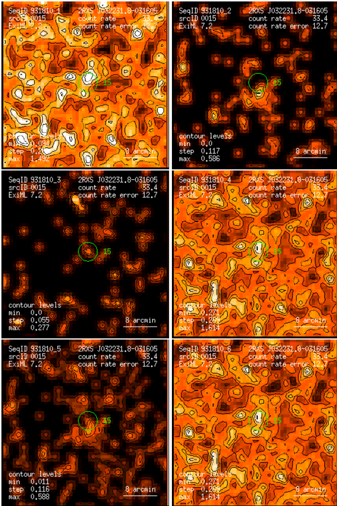
Figure 15: RASS 931810: detection 0015: band rate images, Gaussian filter: (1) PSPC channels 11 – 41, (2) 52 – 90, (3) 91 – 201, (4) 11 – 235, (5) 52 – 201, (6) 11 – 201. Broad band rates in counts/ks. Band rate contour levels in counts/ks/arcmin 2 .
