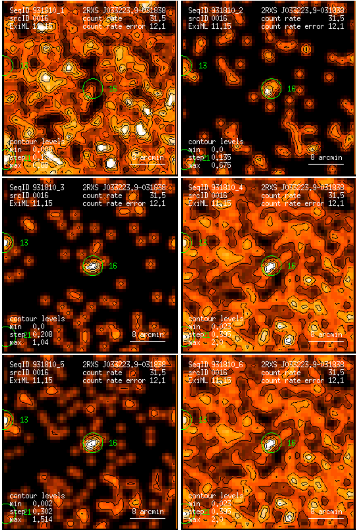
Figure 16: RASS 931810: detection 0016: band rate images, Gaussian filter: (1) PSPC channels 11 – 41, (2) 52 – 90, (3) 91 – 201, (4) 11 – 235, (5) 52 – 201, (6) 11 – 201. Broad band rates in counts/ks. Band rate contour levels in counts/ks/arcmin 2 .
