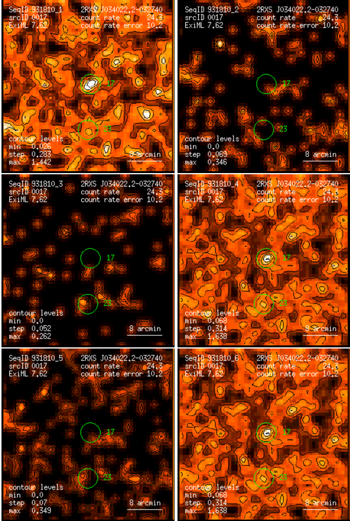
Figure 17: RASS 931810: detection 0017: band rate images, Gaussian filter: (1) PSPC channels 11 – 41, (2) 52 – 90, (3) 91 – 201, (4) 11 – 235, (5) 52 – 201, (6) 11 – 201. Broad band rates in counts/ks. Band rate contour levels in counts/ks/arcmin 2 .
