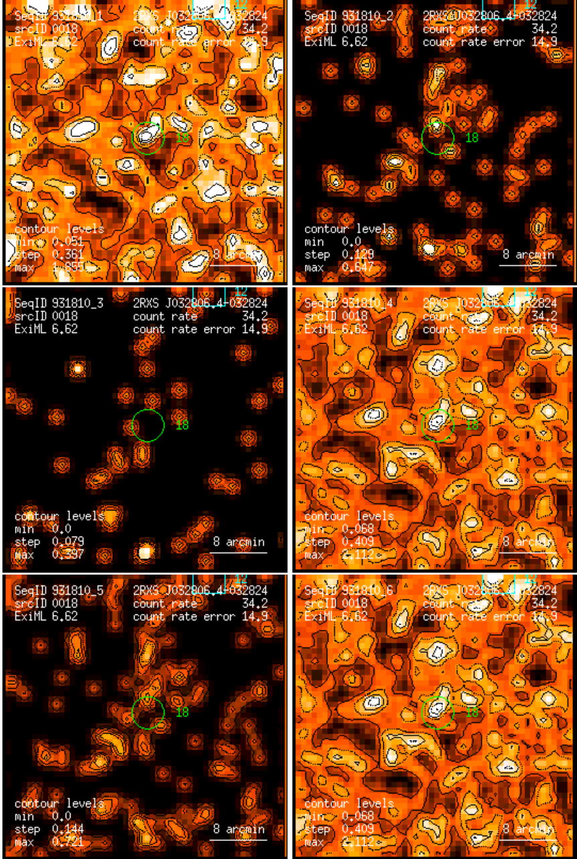
Figure 18: RASS 931810: detection 0018: band rate images, Gaussian filter: (1) PSPC channels 11 – 41, (2) 52 – 90, (3) 91 – 201, (4) 11 – 235, (5) 52 – 201, (6) 11 – 201. Broad band rates in counts/ks. Band rate contour levels in counts/ks/arcmin 2 .
