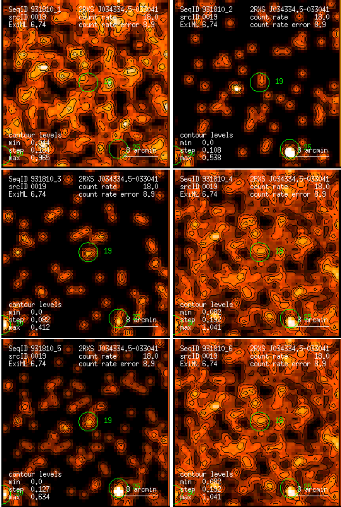
Figure 19: RASS 931810: detection 0019: band rate images, Gaussian filter: (1) PSPC channels 11 – 41, (2) 52 – 90, (3) 91 – 201, (4) 11 – 235, (5) 52 – 201, (6) 11 – 201. Broad band rates in counts/ks. Band rate contour levels in counts/ks/arcmin 2 .
