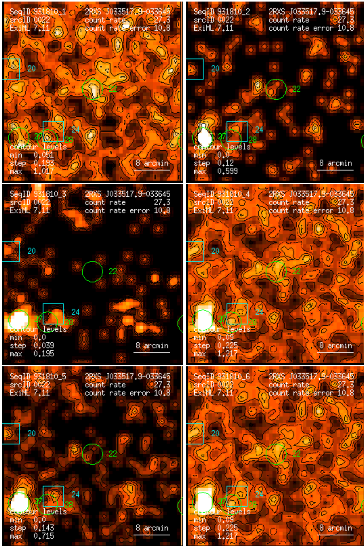
Figure 22: RASS 931810: detection 0022: band rate images, Gaussian filter: (1) PSPC channels 11 – 41, (2) 52 – 90, (3) 91 – 201, (4) 11 – 235, (5) 52 – 201, (6) 11 – 201. Broad band rates in counts/ks. Band rate contour levels in counts/ks/arcmin 2 .
