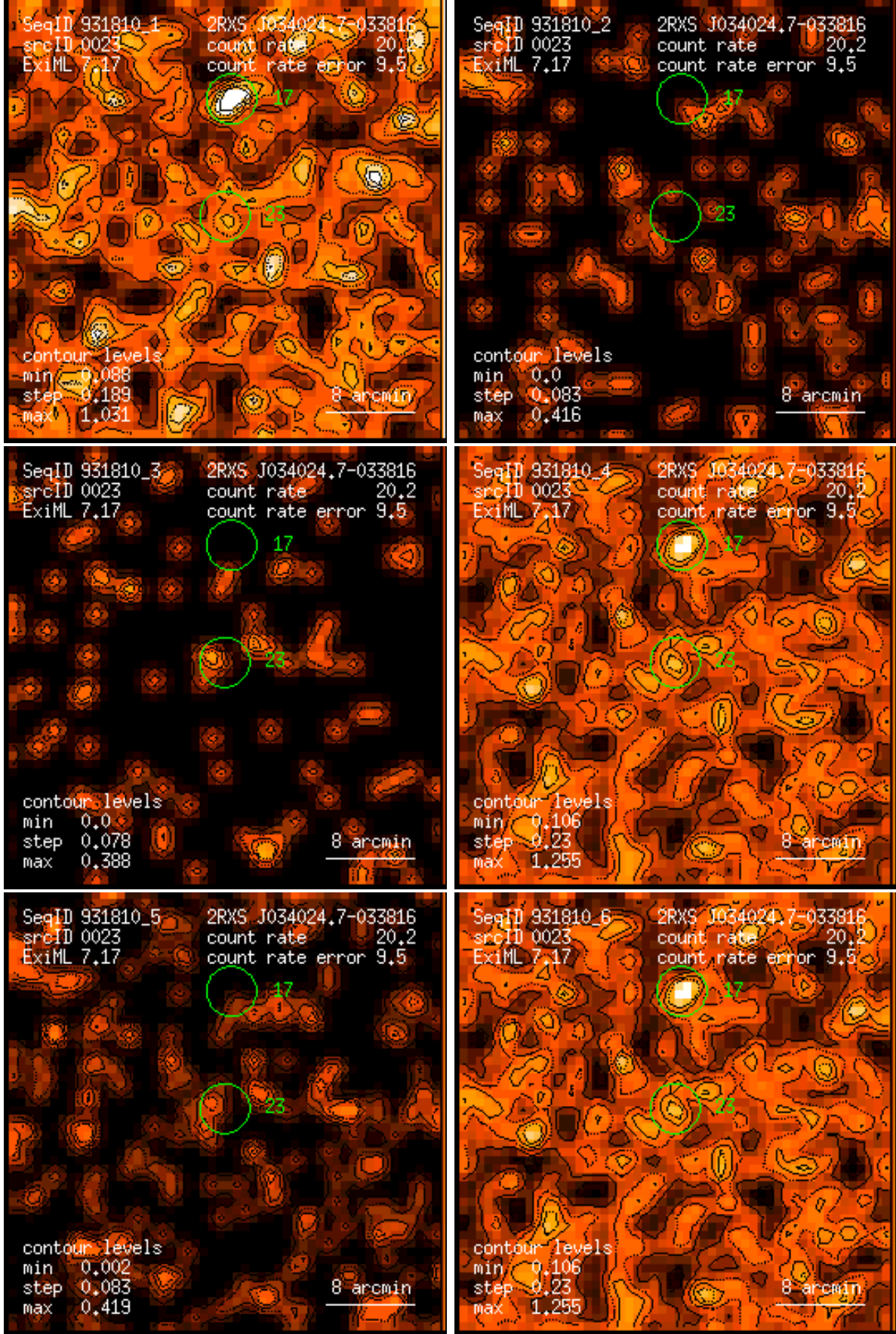
Figure 23: RASS 931810: detection 0023: band rate images, Gaussian filter: (1) PSPC channels 11 – 41, (2) 52 – 90, (3) 91 – 201, (4) 11 – 235, (5) 52 – 201, (6) 11 – 201. Broad band rates in counts/ks. Band rate contour levels in counts/ks/arcmin 2 .
