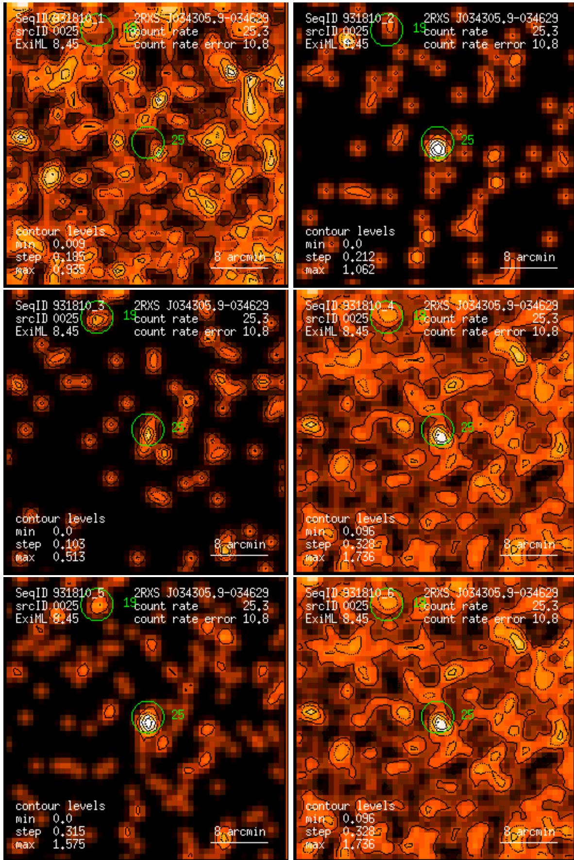
Figure 25: RASS 931810: detection 0025: band rate images, Gaussian filter: (1) PSPC channels 11 – 41, (2) 52 – 90, (3) 91 – 201, (4) 11 – 235, (5) 52 – 201, (6) 11 – 201. Broad band rates in counts/ks. Band rate contour levels in counts/ks/arcmin 2 .
