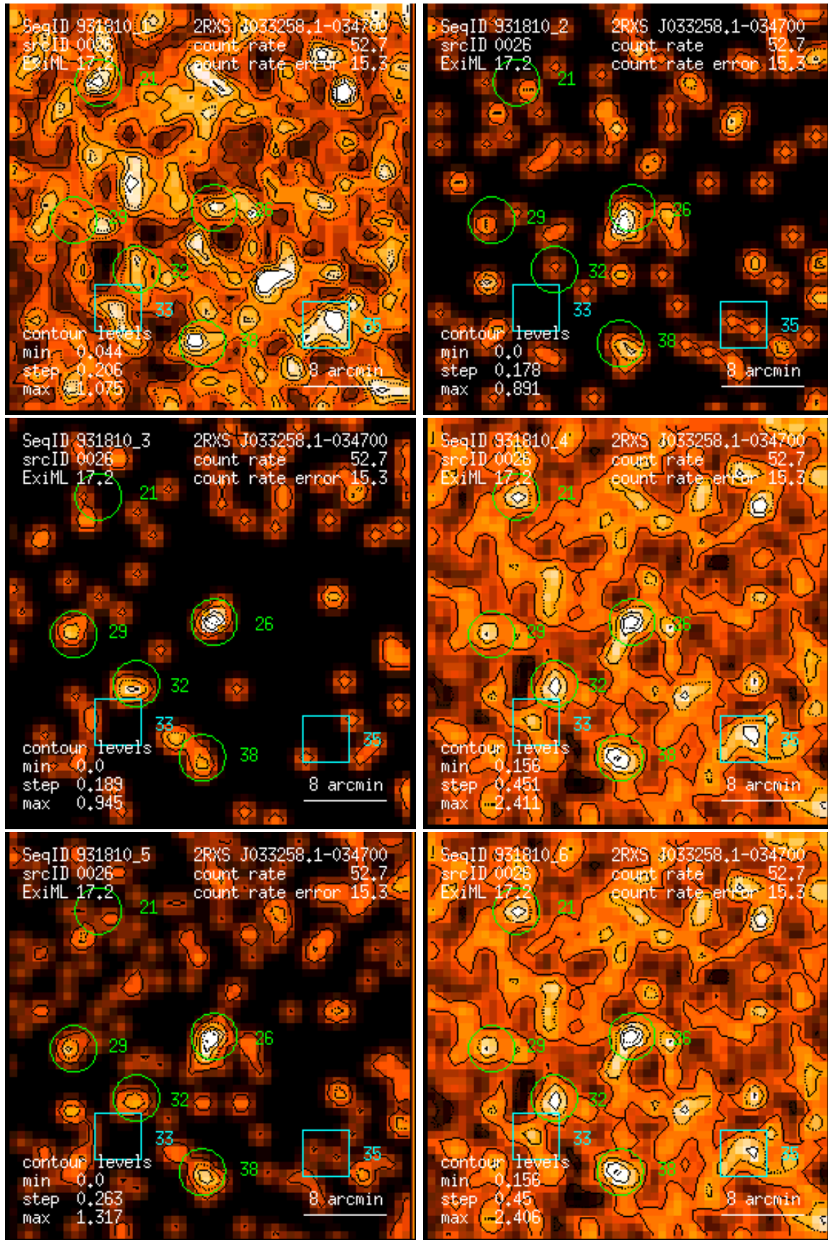
Figure 26: RASS 931810: detection 0026: band rate images, Gaussian filter: (1) PSPC channels 11 – 41, (2) 52 – 90, (3) 91 – 201, (4) 11 – 235, (5) 52 – 201, (6) 11 – 201. Broad band rates in counts/ks. Band rate contour levels in counts/ks/arcmin 2 .
