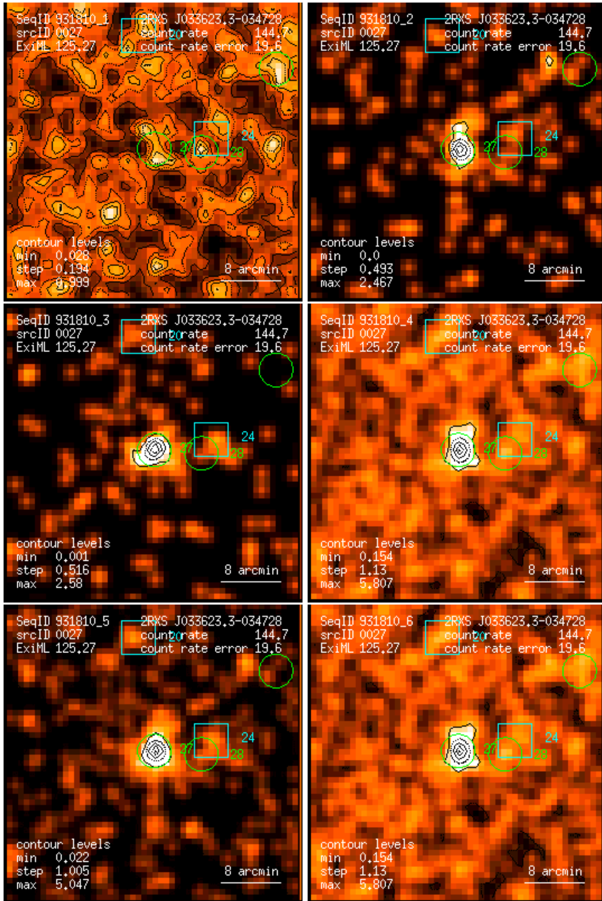
Figure 27: RASS 931810: detection 0027: band rate images, Gaussian filter: (1) PSPC channels 11 – 41, (2) 52 – 90, (3) 91 – 201, (4) 11 – 235, (5) 52 – 201, (6) 11 – 201. Broad band rates in counts/ks. Band rate contour levels in counts/ks/arcmin 2 .
