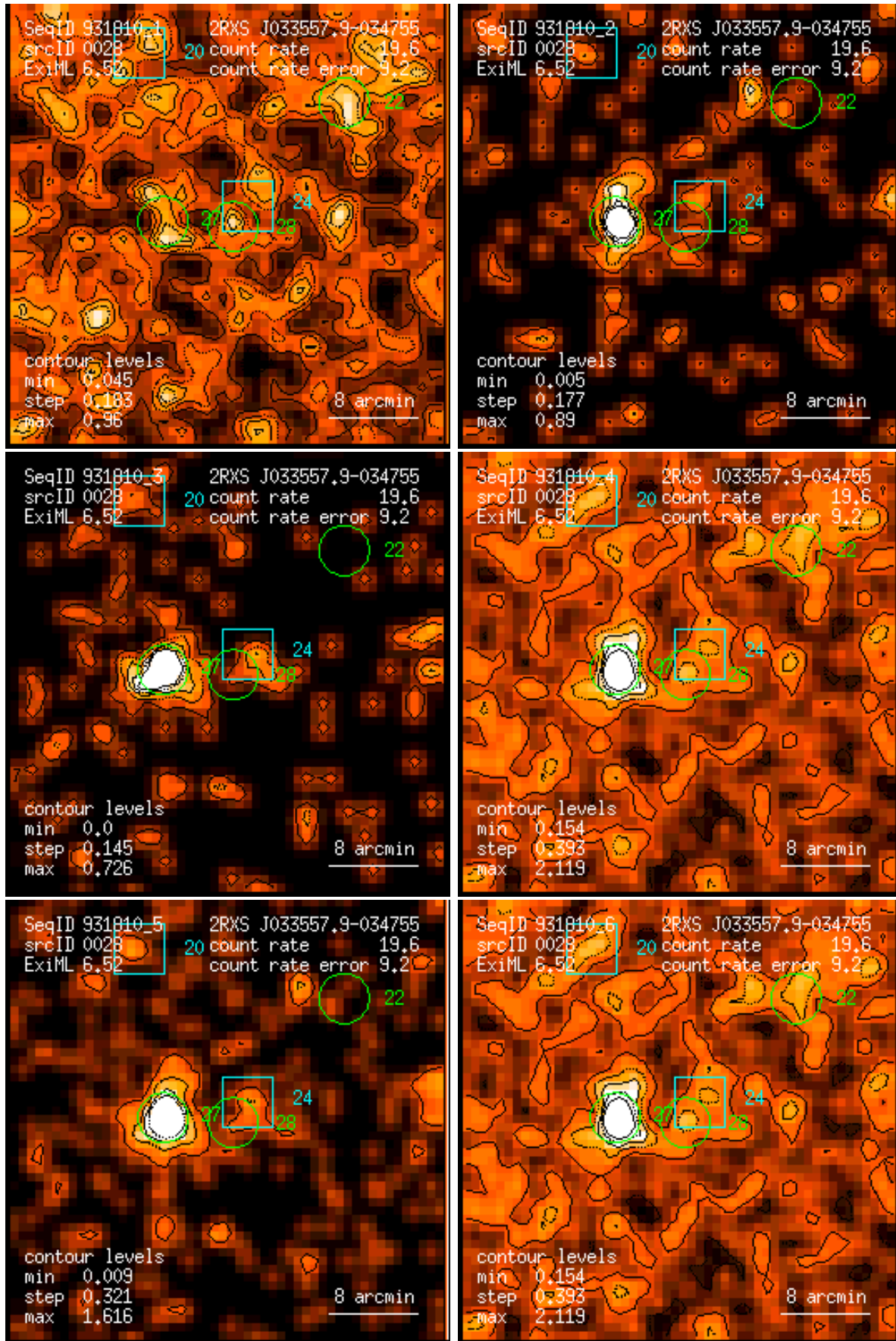
Figure 28: RASS 931810: detection 0028: band rate images, Gaussian filter: (1) PSPC channels 11 – 41, (2) 52 – 90, (3) 91 – 201, (4) 11 – 235, (5) 52 – 201, (6) 11 – 201. Broad band rates in counts/ks. Band rate contour levels in counts/ks/arcmin 2 .
