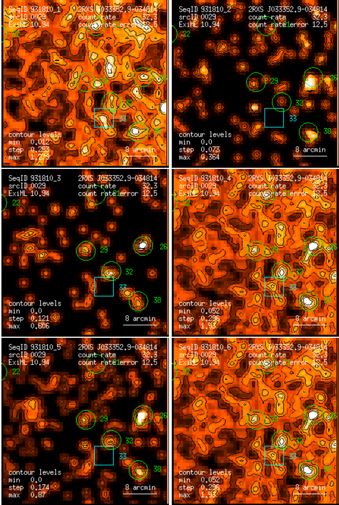
Figure 29: RASS 931810: detection 0029: band rate images, Gaussian filter: (1) PSPC channels 11 – 41, (2) 52 – 90, (3) 91 – 201, (4) 11 – 235, (5) 52 – 201, (6) 11 – 201. Broad band rates in counts/ks. Band rate contour levels in counts/ks/arcmin 2 .
