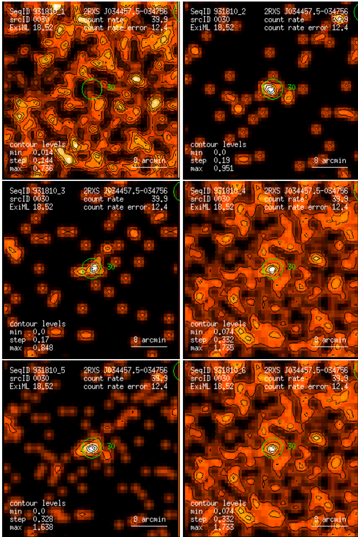
Figure 30: RASS 931810: detection 0030: band rate images, Gaussian filter: (1) PSPC channels 11 – 41, (2) 52 – 90, (3) 91 – 201, (4) 11 – 235, (5) 52 – 201, (6) 11 – 201. Broad band rates in counts/ks. Band rate contour levels in counts/ks/arcmin 2 .
