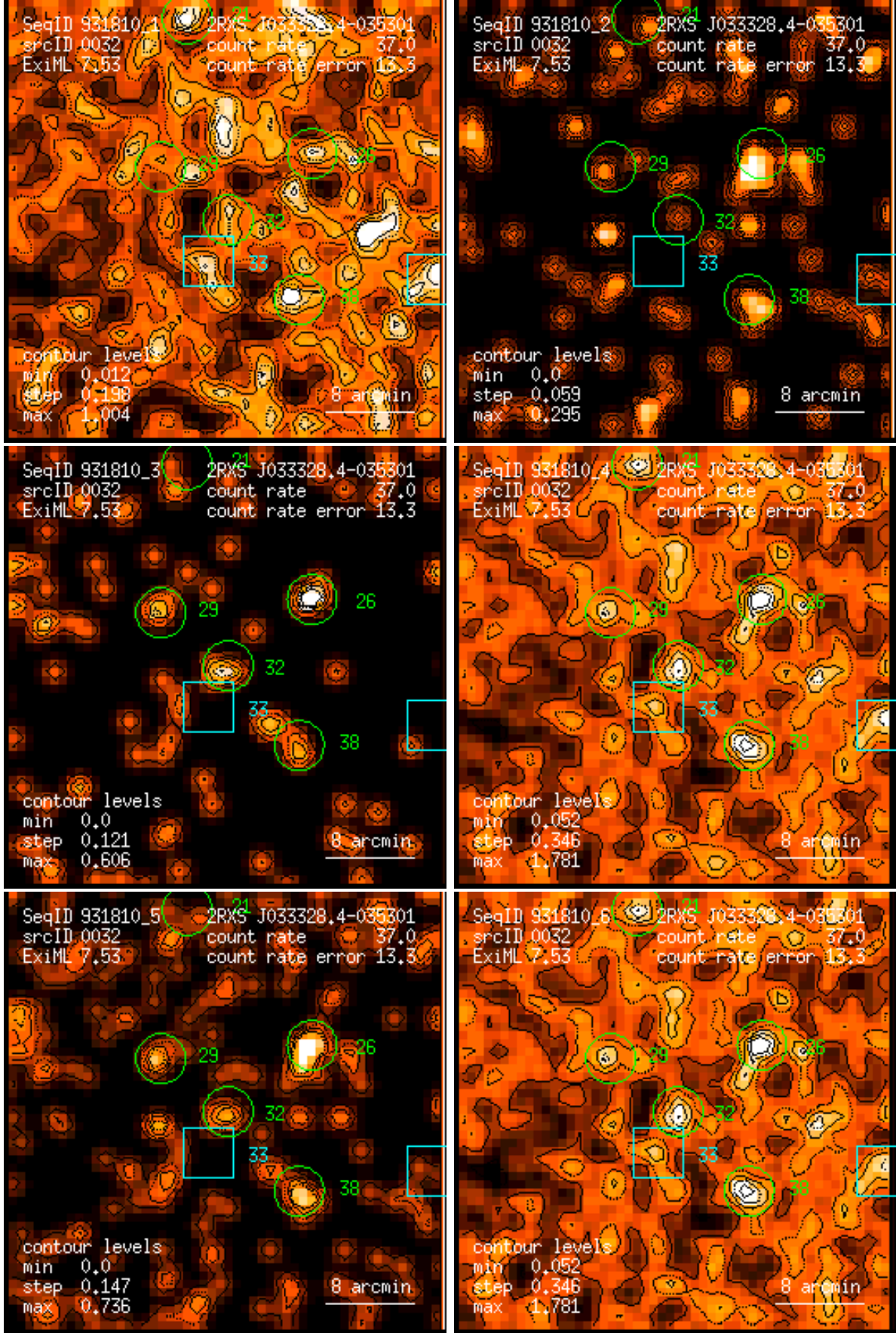
Figure 32: RASS 931810: detection 0032: band rate images, Gaussian filter: (1) PSPC channels 11 – 41, (2) 52 – 90, (3) 91 – 201, (4) 11 – 235, (5) 52 – 201, (6) 11 – 201. Broad band rates in counts/ks. Band rate contour levels in counts/ks/arcmin 2 .
