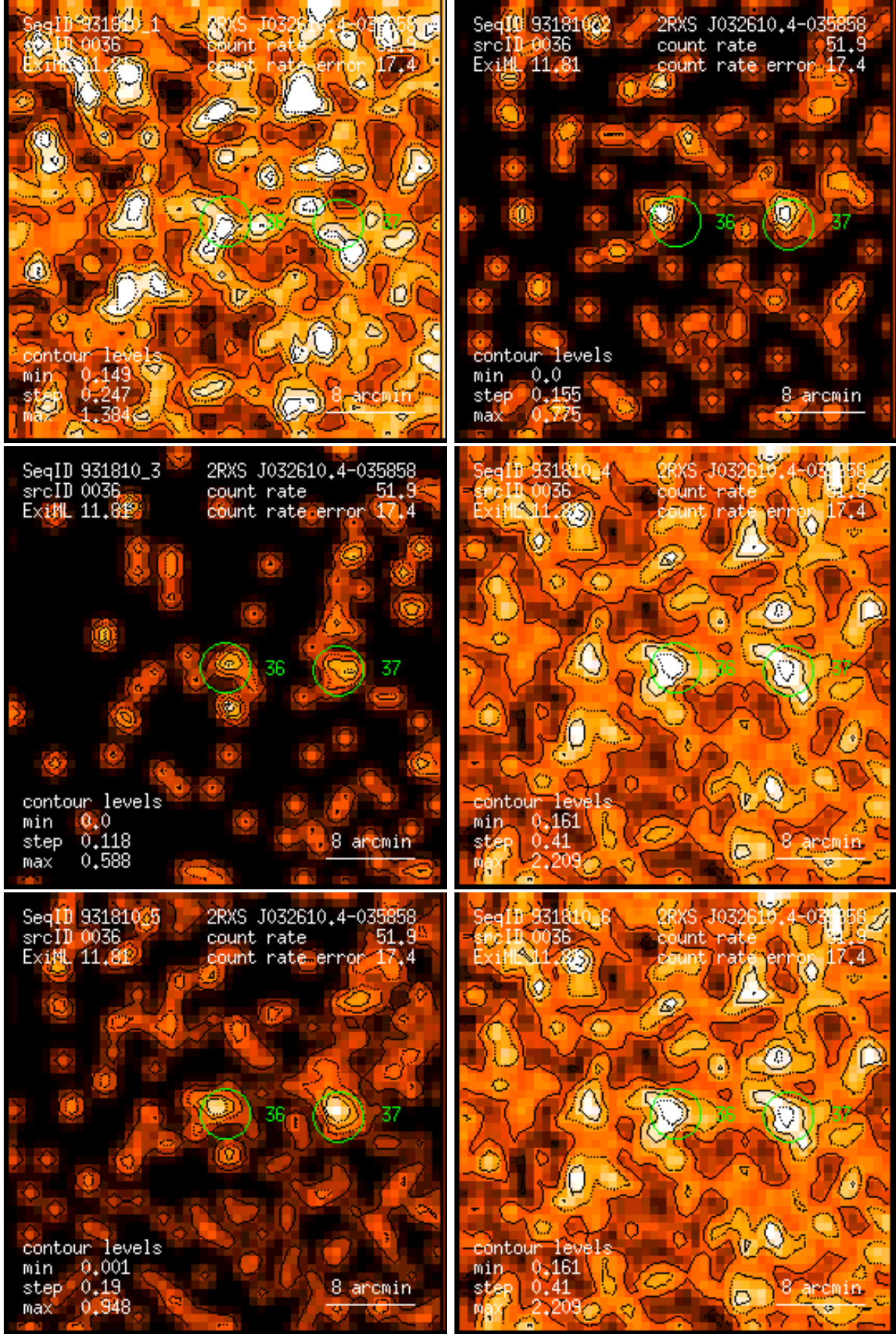
Figure 36: RASS 931810: detection 0036: band rate images, Gaussian filter: (1) PSPC channels 11 – 41, (2) 52 – 90, (3) 91 – 201, (4) 11 – 235, (5) 52 – 201, (6) 11 – 201. Broad band rates in counts/ks. Band rate contour levels in counts/ks/arcmin 2 .
