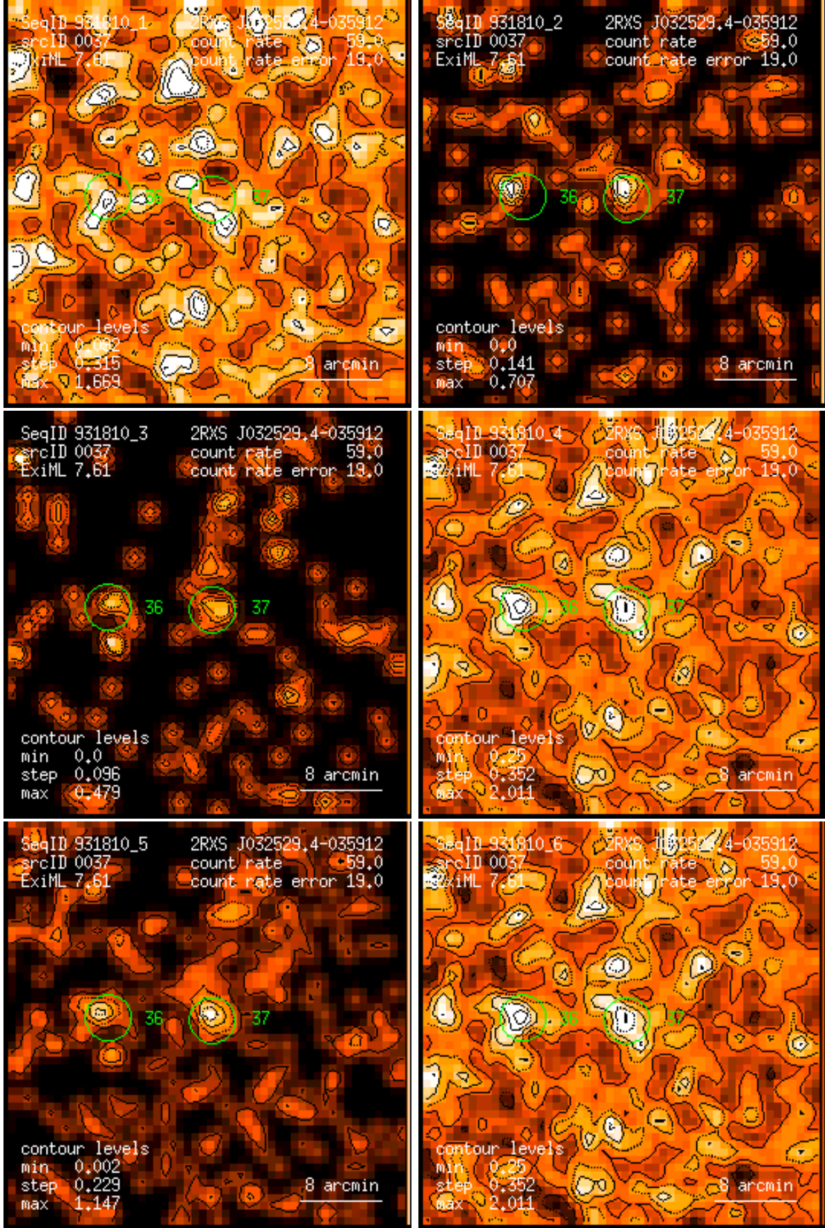
Figure 37: RASS 931810: detection 0037: band rate images, Gaussian filter: (1) PSPC channels 11 – 41, (2) 52 – 90, (3) 91 – 201, (4) 11 – 235, (5) 52 – 201, (6) 11 – 201. Broad band rates in counts/ks. Band rate contour levels in counts/ks/arcmin 2 .
