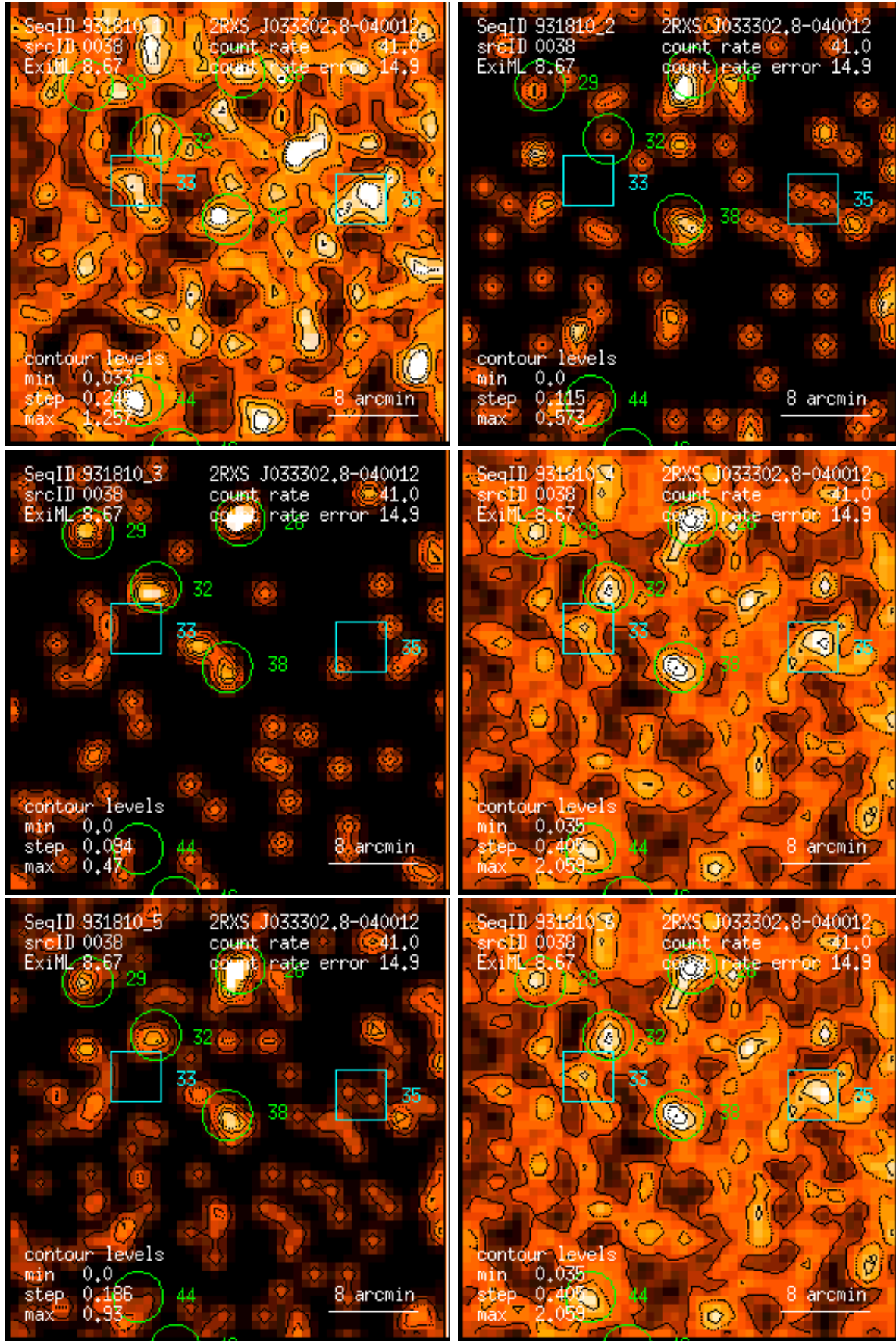
Figure 38: RASS 931810: detection 0038: band rate images, Gaussian filter: (1) PSPC channels 11 – 41, (2) 52 – 90, (3) 91 – 201, (4) 11 – 235, (5) 52 – 201, (6) 11 – 201. Broad band rates in counts/ks. Band rate contour levels in counts/ks/arcmin 2 .
