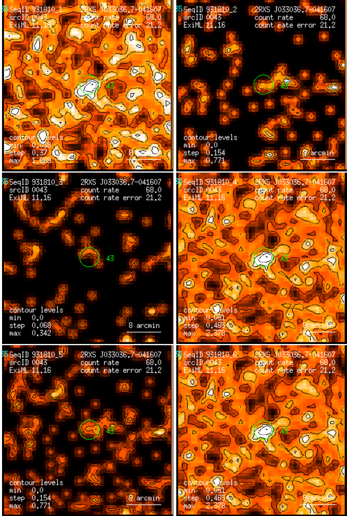
Figure 43: RASS 931810: detection 0043: band rate images, Gaussian filter: (1) PSPC channels 11 – 41, (2) 52 – 90, (3) 91 – 201, (4) 11 – 235, (5) 52 – 201, (6) 11 – 201. Broad band rates in counts/ks. Band rate contour levels in counts/ks/arcmin 2 .
