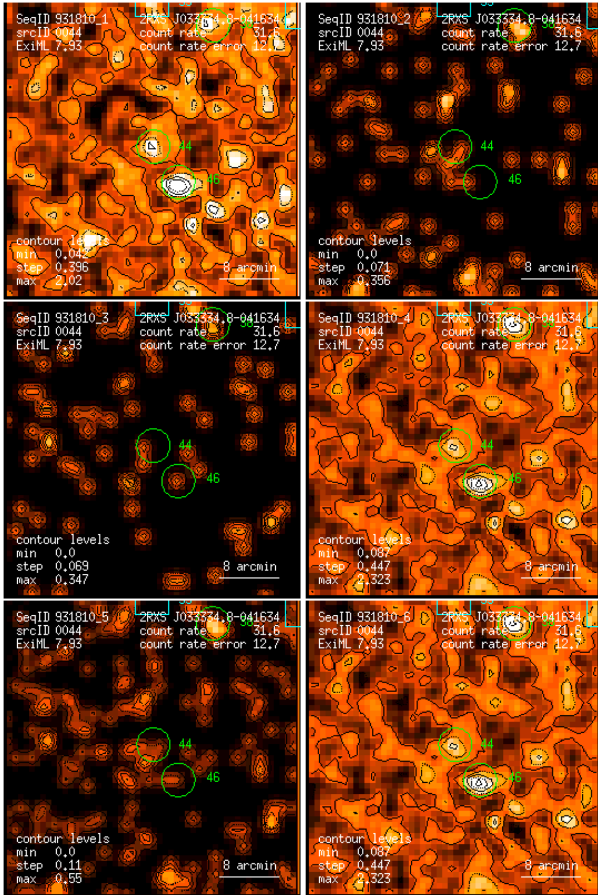
Figure 44: RASS 931810: detection 0044: band rate images, Gaussian filter: (1) PSPC channels 11 – 41, (2) 52 – 90, (3) 91 – 201, (4) 11 – 235, (5) 52 – 201, (6) 11 – 201. Broad band rates in counts/ks. Band rate contour levels in counts/ks/arcmin 2 .
