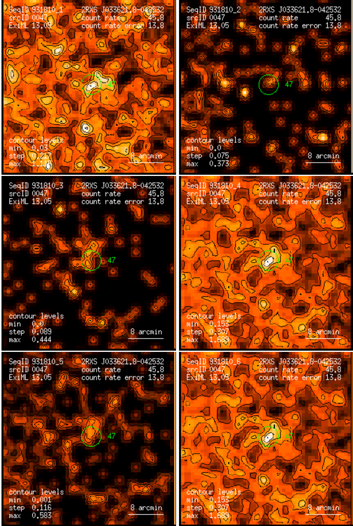
Figure 47: RASS 931810: detection 0047: band rate images, Gaussian filter: (1) PSPC channels 11 – 41, (2) 52 – 90, (3) 91 – 201, (4) 11 – 235, (5) 52 – 201, (6) 11 – 201. Broad band rates in counts/ks. Band rate contour levels in counts/ks/arcmin 2 .
