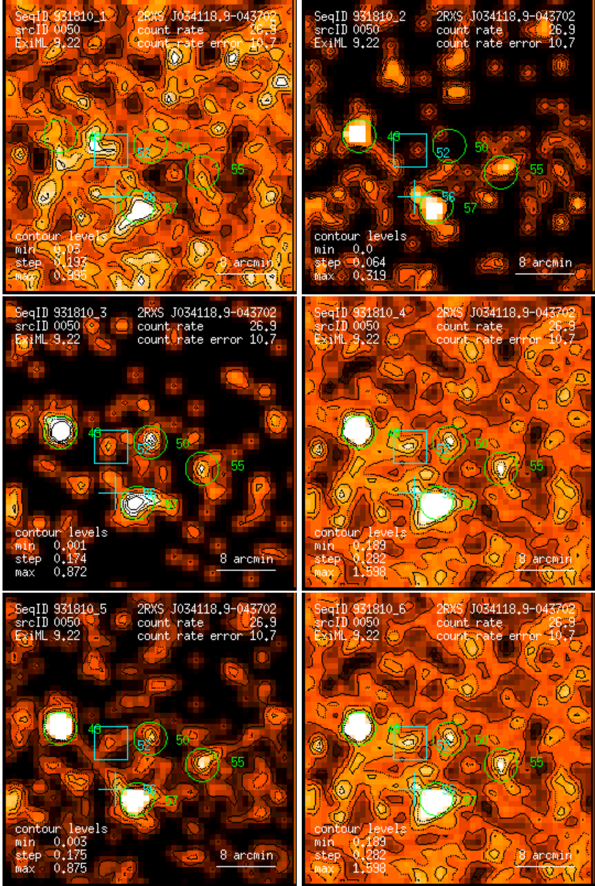
Figure 50: RASS 931810: detection 0050: band rate images, Gaussian filter: (1) PSPC channels 11 – 41, (2) 52 – 90, (3) 91 – 201, (4) 11 – 235, (5) 52 – 201, (6) 11 – 201. Broad band rates in counts/ks. Band rate contour levels in counts/ks/arcmin 2 .
