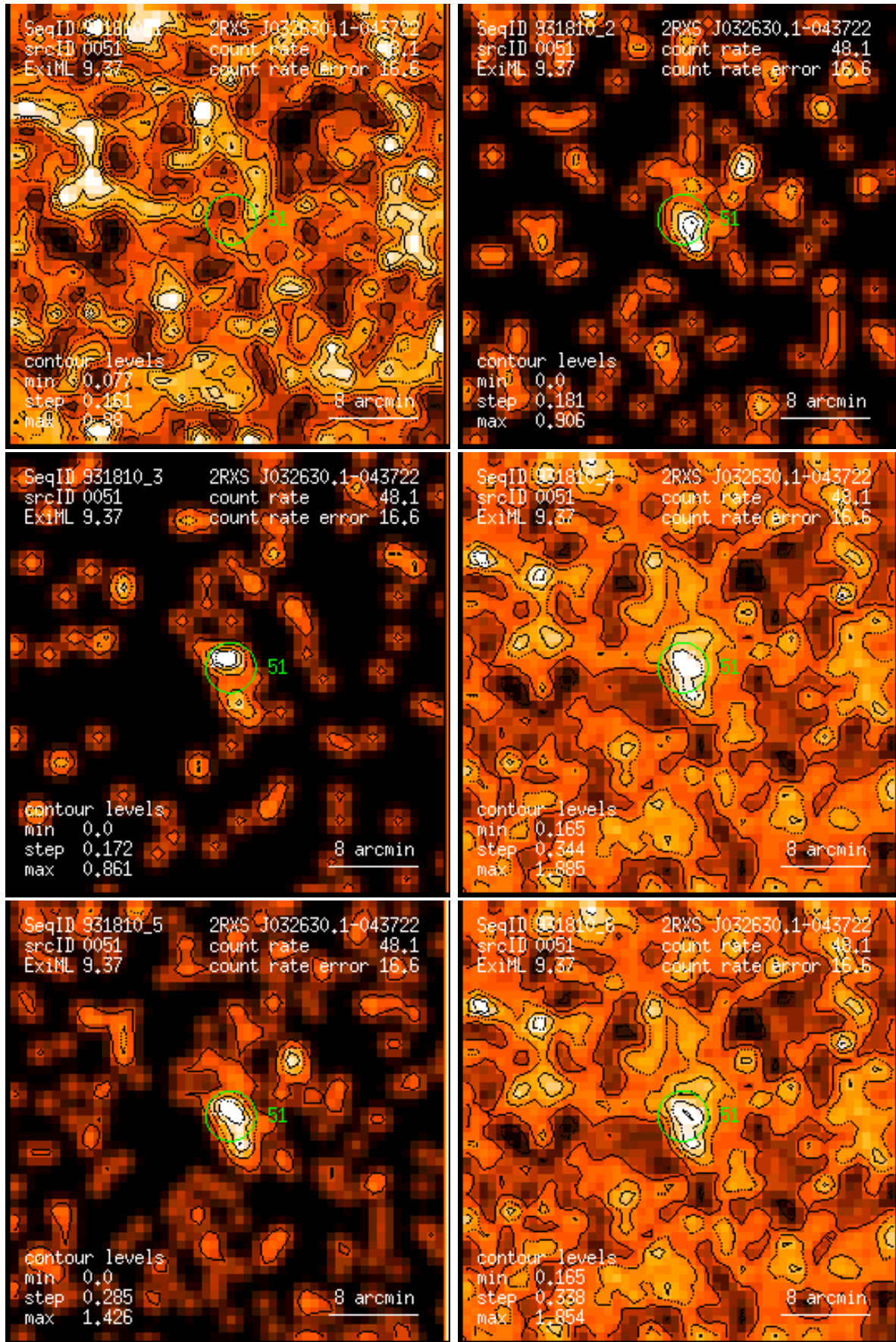
Figure 51: RASS 931810: detection 0051: band rate images, Gaussian filter: (1) PSPC channels 11 – 41, (2) 52 – 90, (3) 91 – 201, (4) 11 – 235, (5) 52 – 201, (6) 11 – 201. Broad band rates in counts/ks. Band rate contour levels in counts/ks/arcmin 2 .
