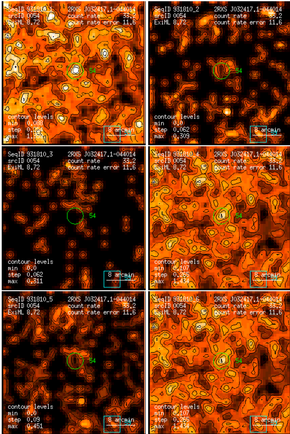
Figure 54: RASS 931810: detection 0054: band rate images, Gaussian filter: (1) PSPC channels 11 – 41, (2) 52 – 90, (3) 91 – 201, (4) 11 – 235, (5) 52 – 201, (6) 11 – 201. Broad band rates in counts/ks. Band rate contour levels in counts/ks/arcmin 2 .
