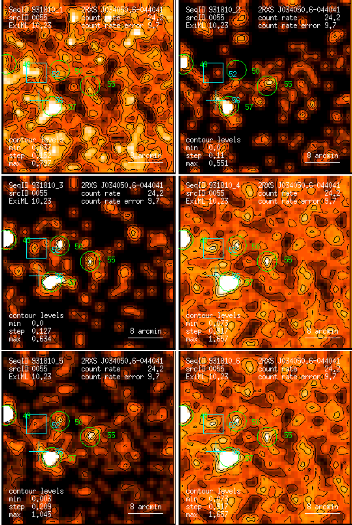
Figure 55: RASS 931810: detection 0055: band rate images, Gaussian filter: (1) PSPC channels 11 – 41, (2) 52 – 90, (3) 91 – 201, (4) 11 – 235, (5) 52 – 201, (6) 11 – 201. Broad band rates in counts/ks. Band rate contour levels in counts/ks/arcmin 2 .
