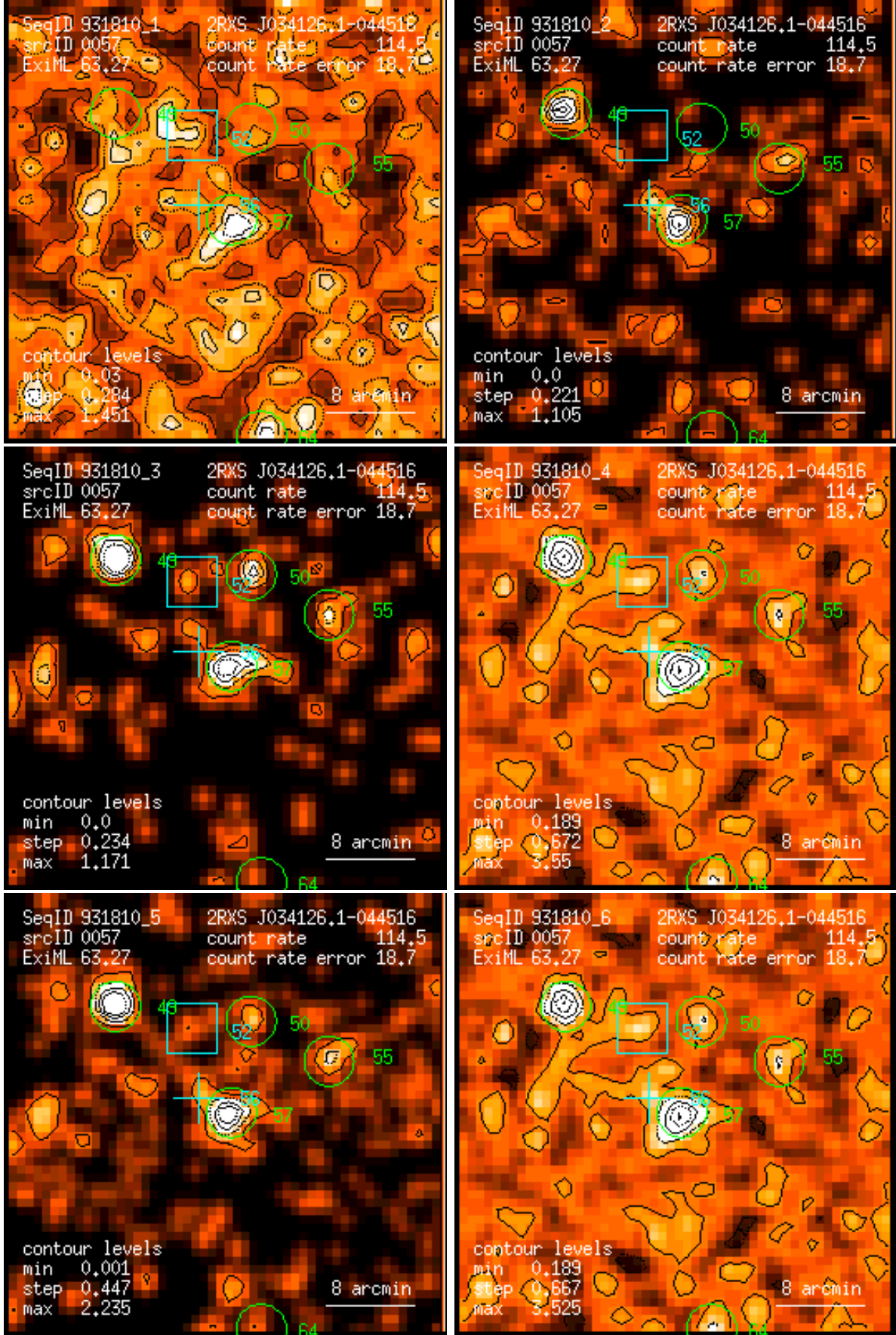
Figure 57: RASS 931810: detection 0057: band rate images, Gaussian filter: (1) PSPC channels 11 – 41, (2) 52 – 90, (3) 91 – 201, (4) 11 – 235, (5) 52 – 201, (6) 11 – 201. Broad band rates in counts/ks. Band rate contour levels in counts/ks/arcmin 2 .
