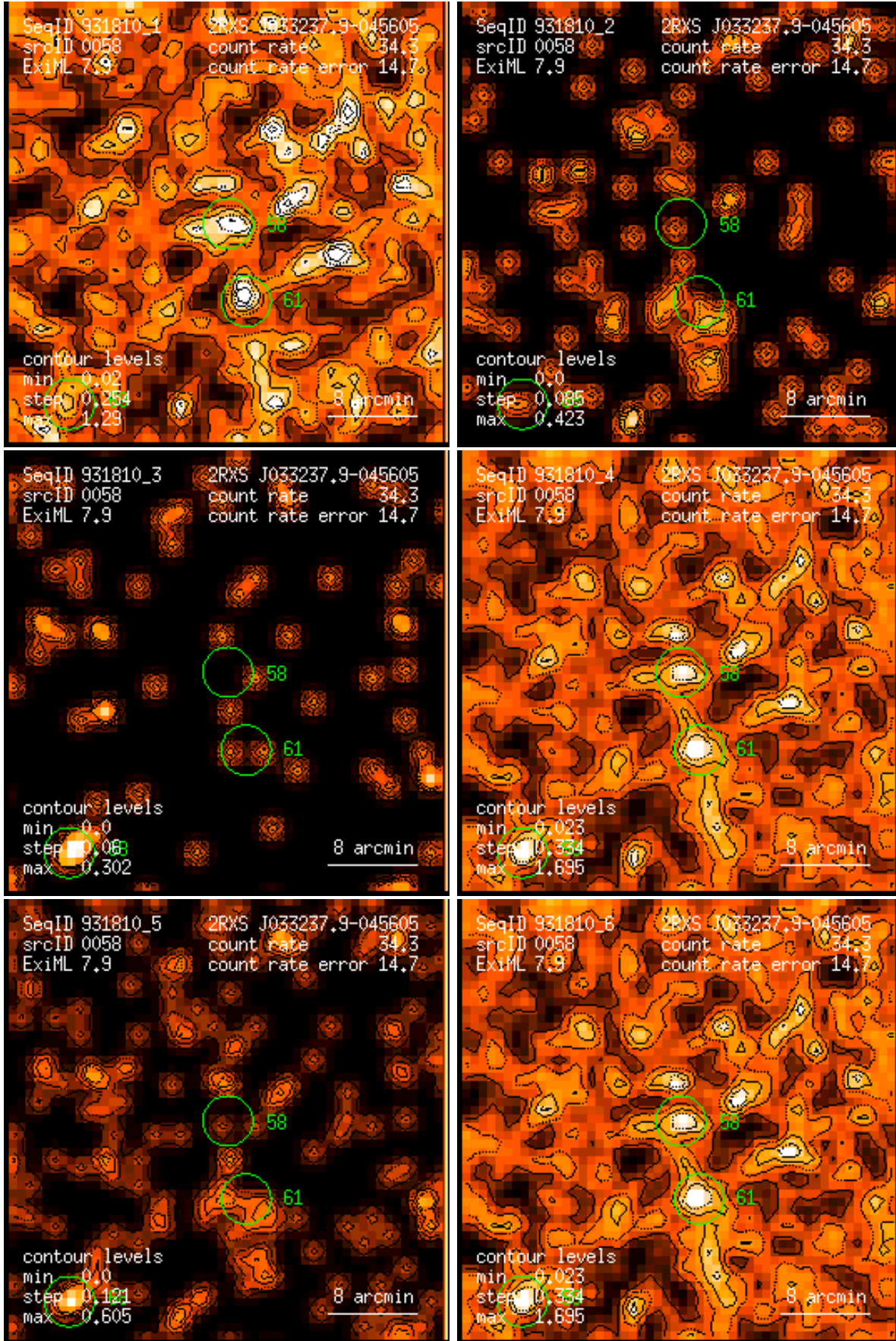
Figure 58: RASS 931810: detection 0058: band rate images, Gaussian filter: (1) PSPC channels 11 – 41, (2) 52 – 90, (3) 91 – 201, (4) 11 – 235, (5) 52 – 201, (6) 11 – 201. Broad band rates in counts/ks. Band rate contour levels in counts/ks/arcmin 2 .
