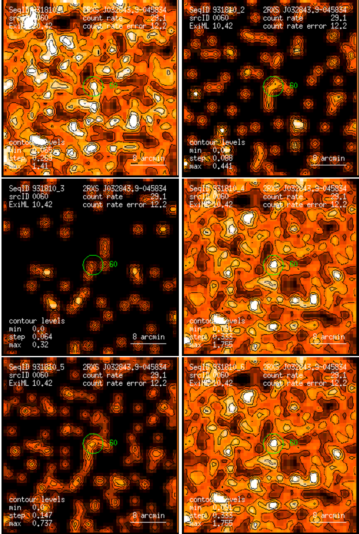
Figure 60: RASS 931810: detection 0060: band rate images, Gaussian filter: (1) PSPC channels 11 – 41, (2) 52 – 90, (3) 91 – 201, (4) 11 – 235, (5) 52 – 201, (6) 11 – 201. Broad band rates in counts/ks. Band rate contour levels in counts/ks/arcmin 2 .
