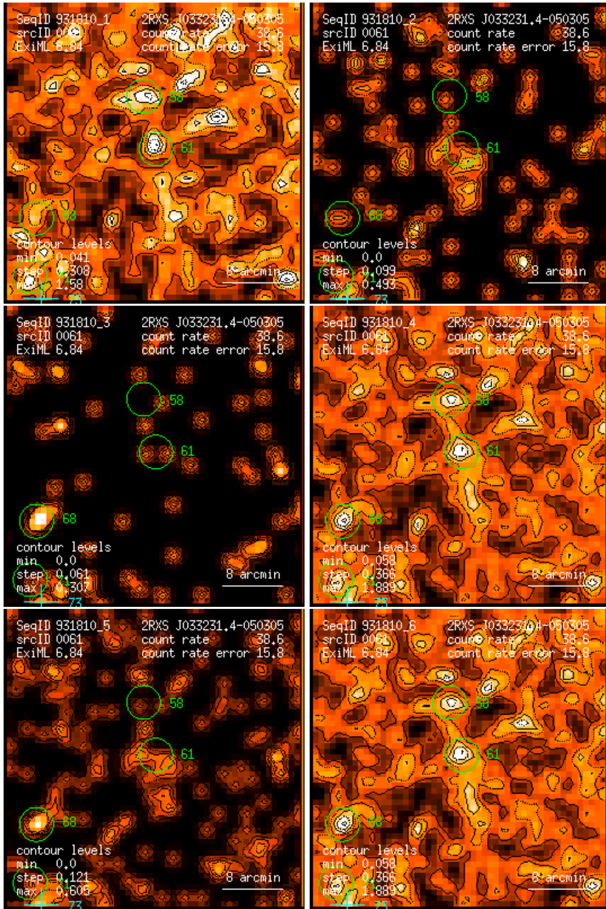
Figure 61: RASS 931810: detection 0061: band rate images, Gaussian filter: (1) PSPC channels 11 – 41, (2) 52 – 90, (3) 91 – 201, (4) 11 – 235, (5) 52 – 201, (6) 11 – 201. Broad band rates in counts/ks. Band rate contour levels in counts/ks/arcmin 2 .
