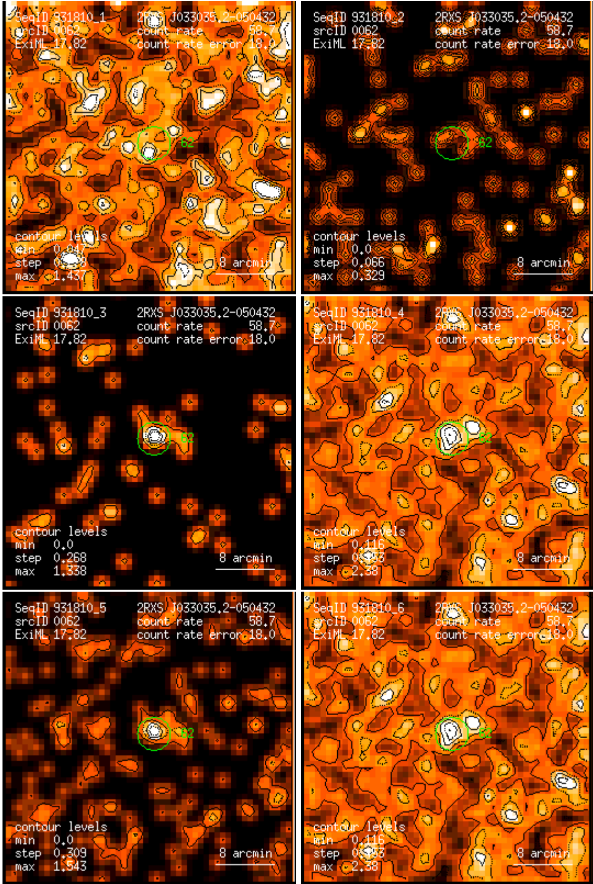
Figure 62: RASS 931810: detection 0062: band rate images, Gaussian filter: (1) PSPC channels 11 – 41, (2) 52 – 90, (3) 91 – 201, (4) 11 – 235, (5) 52 – 201, (6) 11 – 201. Broad band rates in counts/ks. Band rate contour levels in counts/ks/arcmin 2 .
