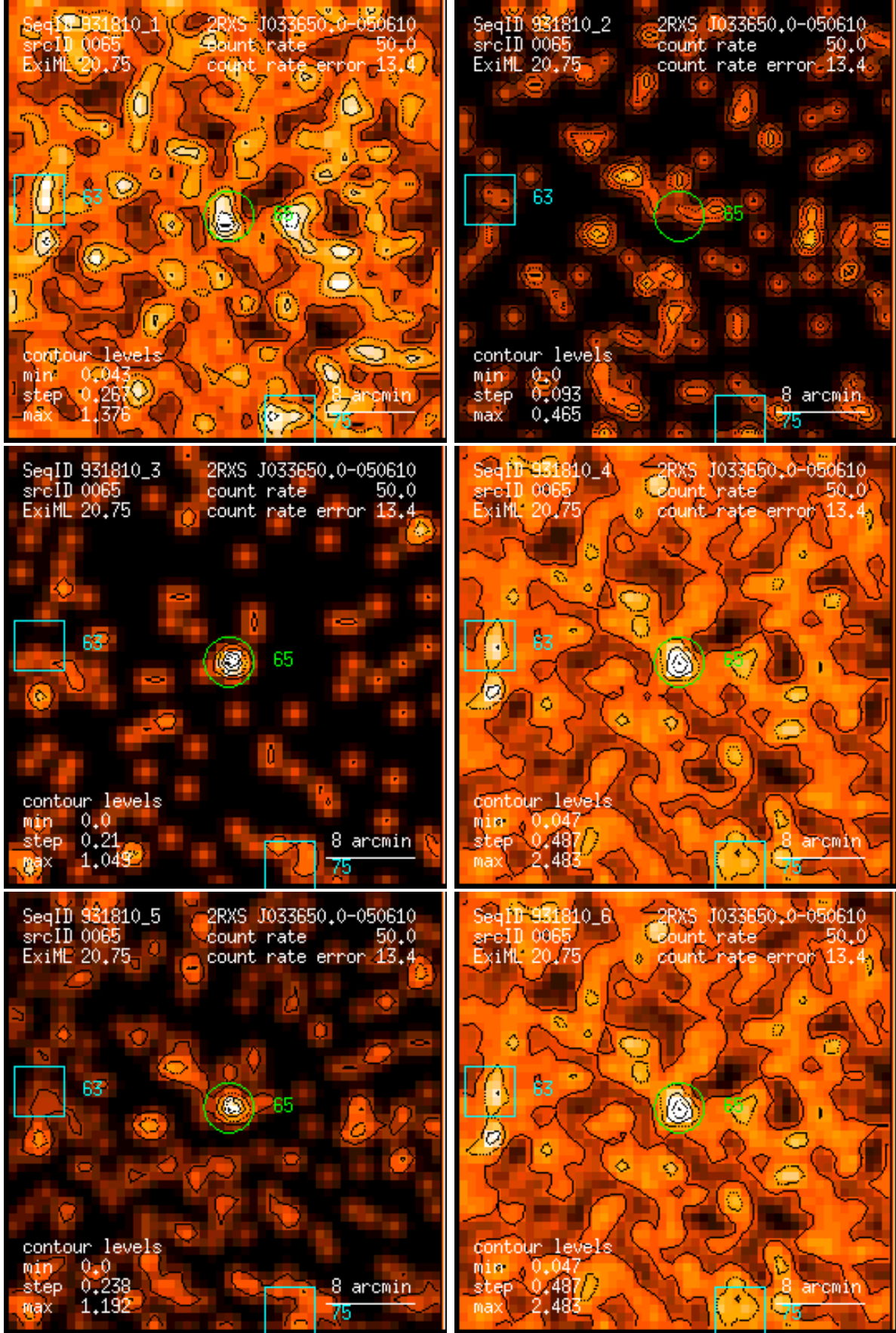
Figure 65: RASS 931810: detection 0065: band rate images, Gaussian filter: (1) PSPC channels 11 – 41, (2) 52 – 90, (3) 91 – 201, (4) 11 – 235, (5) 52 – 201, (6) 11 – 201. Broad band rates in counts/ks. Band rate contour levels in counts/ks/arcmin 2 .
