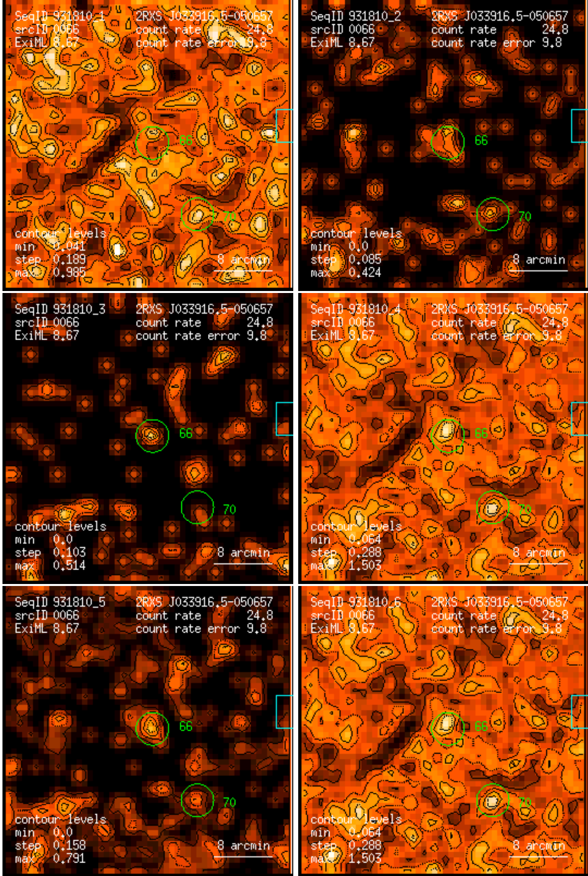
Figure 66: RASS 931810: detection 0066: band rate images, Gaussian filter: (1) PSPC channels 11 – 41, (2) 52 – 90, (3) 91 – 201, (4) 11 – 235, (5) 52 – 201, (6) 11 – 201. Broad band rates in counts/ks. Band rate contour levels in counts/ks/arcmin 2 .
