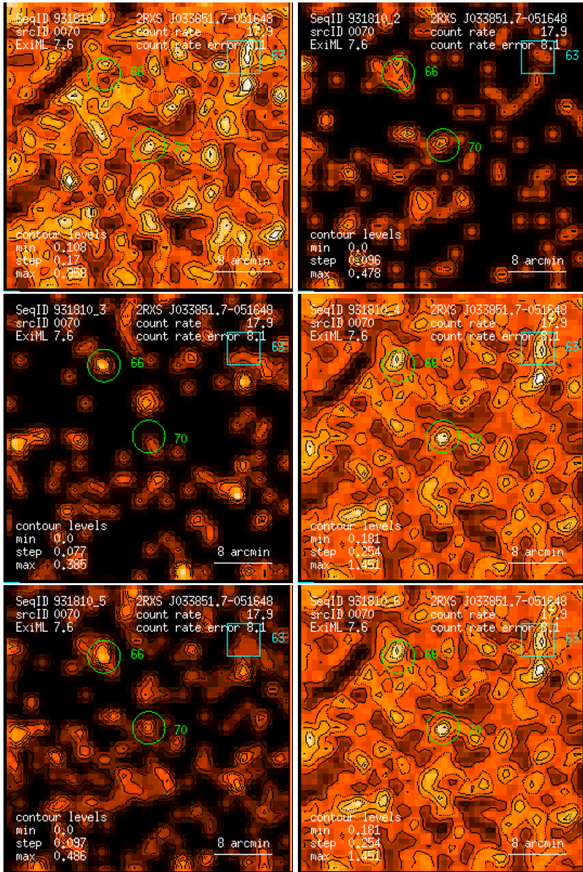
Figure 70: RASS 931810: detection 0070: band rate images, Gaussian filter: (1) PSPC channels 11 – 41, (2) 52 – 90, (3) 91 – 201, (4) 11 – 235, (5) 52 – 201, (6) 11 – 201. Broad band rates in counts/ks. Band rate contour levels in counts/ks/arcmin 2 .
