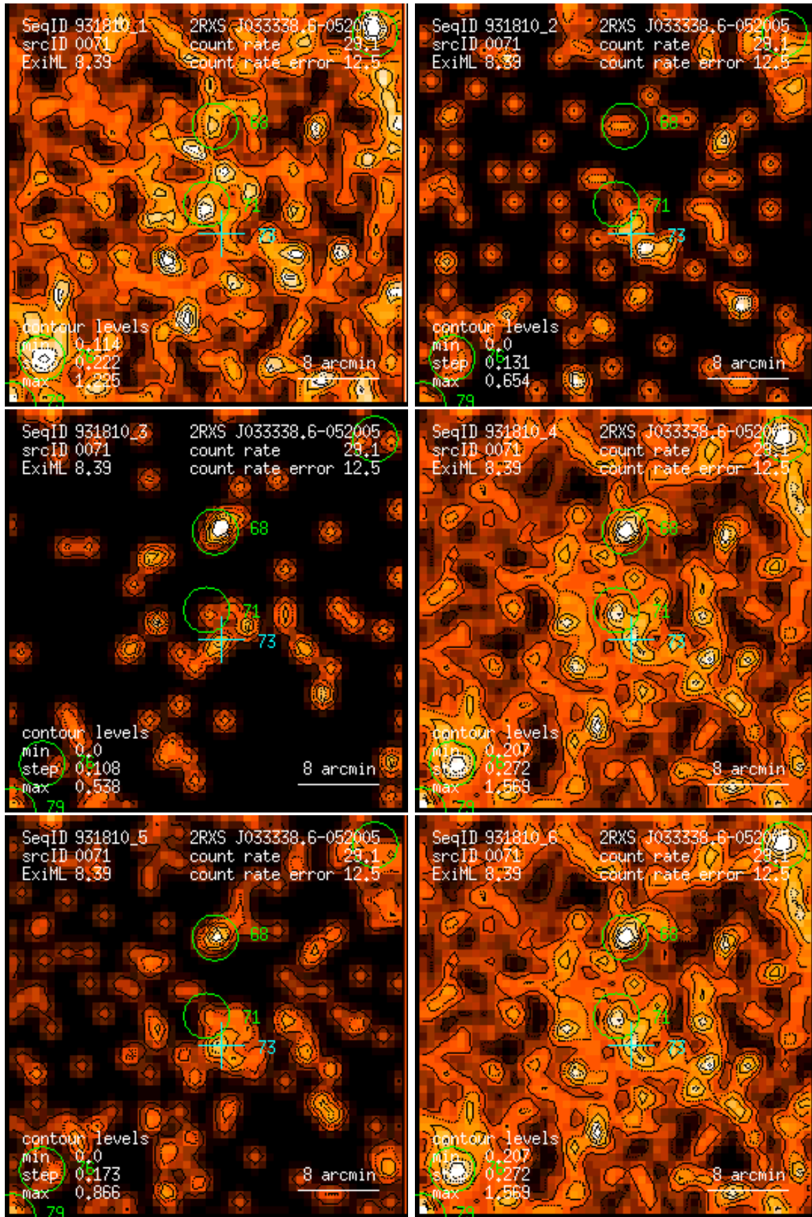
Figure 71: RASS 931810: detection 0071: band rate images, Gaussian filter: (1) PSPC channels 11 – 41, (2) 52 – 90, (3) 91 – 201, (4) 11 – 235, (5) 52 – 201, (6) 11 – 201. Broad band rates in counts/ks. Band rate contour levels in counts/ks/arcmin 2 .
