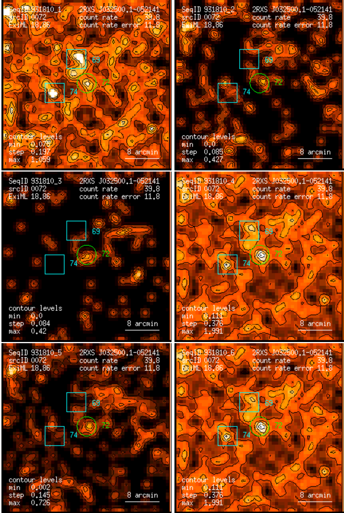
Figure 72: RASS 931810: detection 0072: band rate images, Gaussian filter: (1) PSPC channels 11 – 41, (2) 52 – 90, (3) 91 – 201, (4) 11 – 235, (5) 52 – 201, (6) 11 – 201. Broad band rates in counts/ks. Band rate contour levels in counts/ks/arcmin 2 .
