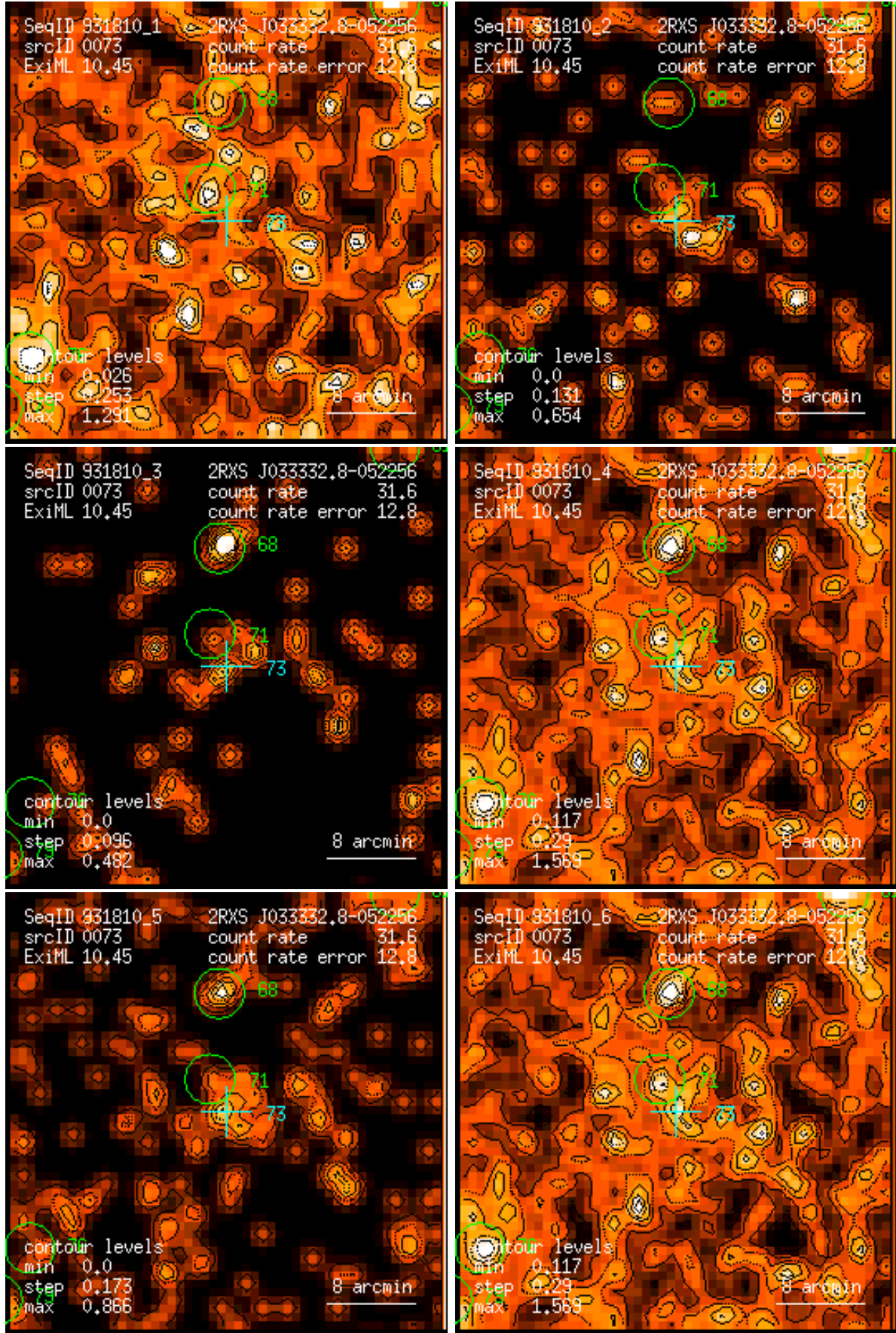
Figure 73: RASS 931810: detection 0073: band rate images, Gaussian filter: (1) PSPC channels 11 – 41, (2) 52 – 90, (3) 91 – 201, (4) 11 – 235, (5) 52 – 201, (6) 11 – 201. Broad band rates in counts/ks. Band rate contour levels in counts/ks/arcmin 2 .
