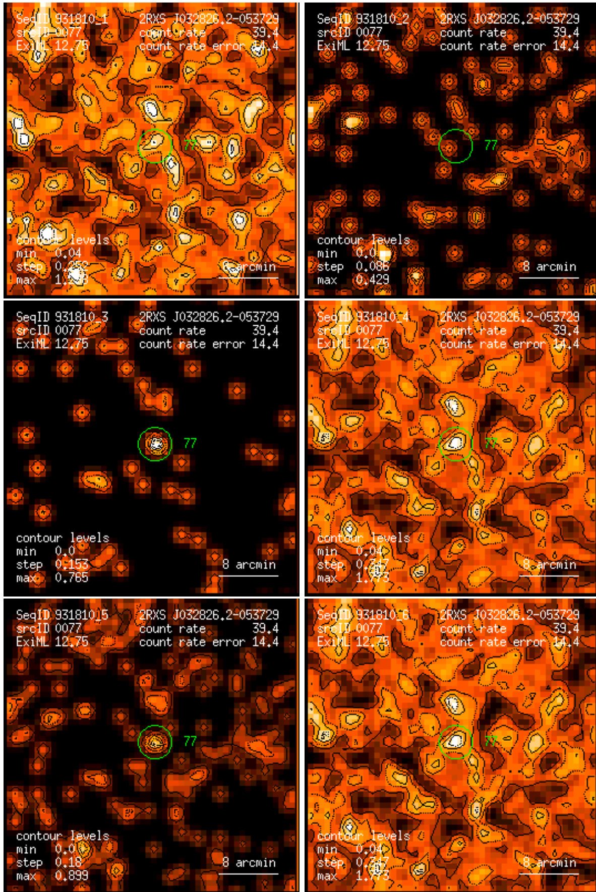
Figure 77: RASS 931810: detection 0077: band rate images, Gaussian filter: (1) PSPC channels 11 – 41, (2) 52 – 90, (3) 91 – 201, (4) 11 – 235, (5) 52 – 201, (6) 11 – 201. Broad band rates in counts/ks. Band rate contour levels in counts/ks/arcmin 2 .
