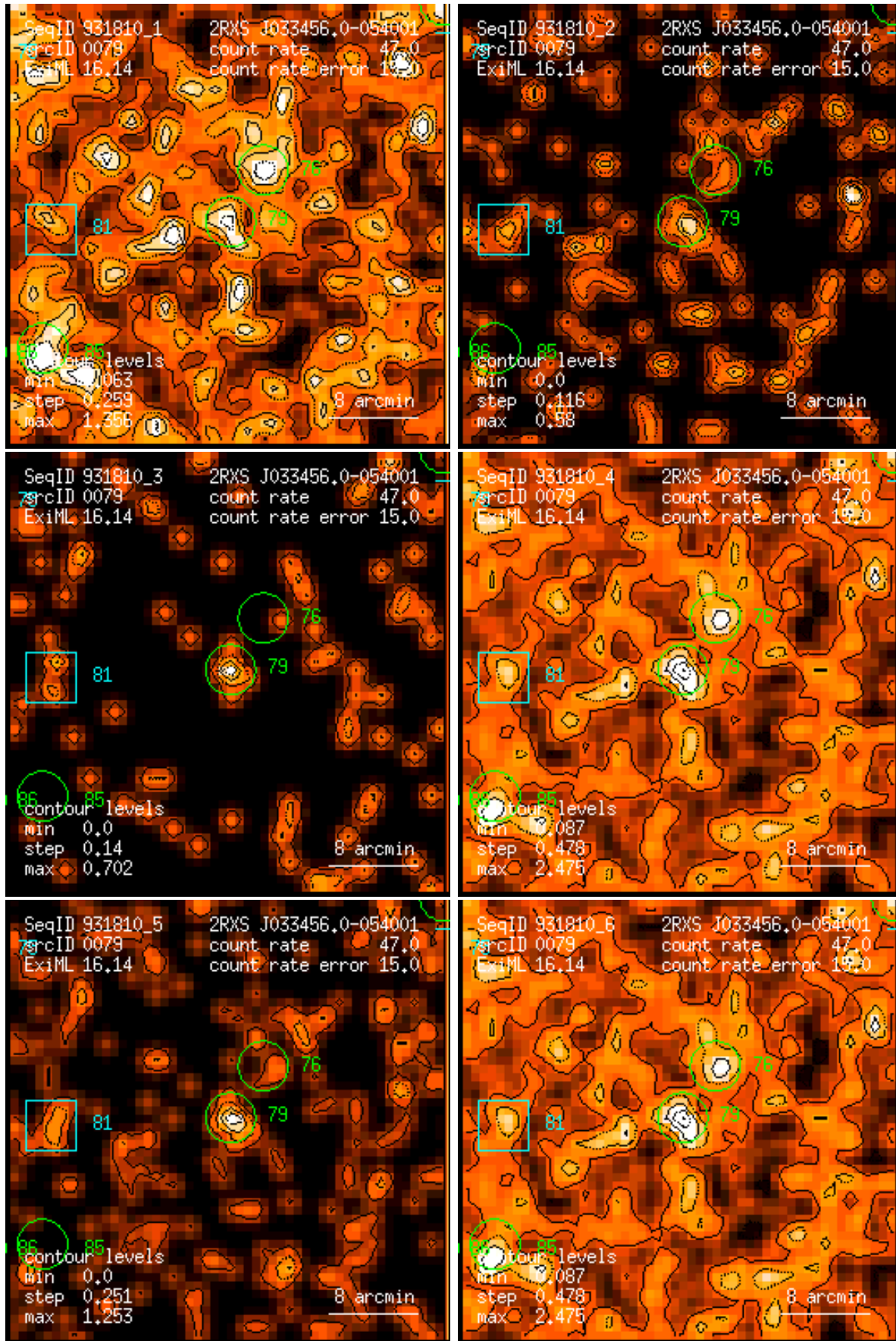
Figure 79: RASS 931810: detection 0079: band rate images, Gaussian filter: (1) PSPC channels 11 – 41, (2) 52 – 90, (3) 91 – 201, (4) 11 – 235, (5) 52 – 201, (6) 11 – 201. Broad band rates in counts/ks. Band rate contour levels in counts/ks/arcmin 2 .
